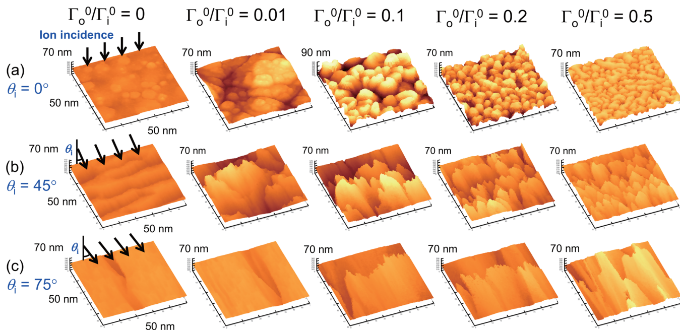
FIG. 9. (Color online) Surface features of Si at t=60 s after the start of etching in \text{Cl}_2/\text{O}_2 plasma, simulated in the presence of incoming oxygen fluxes from the plasma ( \Gamma_o^0 \neq 0 ) with ion incidence angles of \theta_i = (a) 0^\circ , (b) 45^\circ , and (c) 75^\circ . The oxygen-to-ion flux ratio concerned is in the range \Gamma_o^0/\Gamma_i^0 = 0-0.5 , and the other calculation conditions in the ASCeM-3D are the same as those of Fig. 3 ( E_i = 100 eV, \Gamma_n^0/\Gamma_i^0 = 100 , \Gamma_p^0 = 0 ). Note that the surface features for \Gamma_o^0/\Gamma_i^0 = 0 of interest here are the same as those shown at t=60 s in Figs. 3(a), 3(d), and 3(f).
