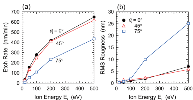
Fig. 6. (Color online) (a) Etch rate and (b) rms surface roughness at t = 60 s as a function of ion energy in the range E_i = 20 –500 eV with ion incidence angles of \theta_i = 0^\circ , 45^\circ , and 75^\circ derived from the simulations of Fig. 5.
