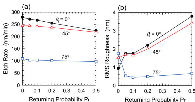
FIG. 12. (Color online) (a) Etch rate and (b) rms surface roughness at t = 60 s as a function of returning probability in the range P_r = 0 – 0.5 with ion incidence angles of \theta_i = 0^\circ, 45^\circ , and 75^\circ derived from the simulations of Fig. 11.
