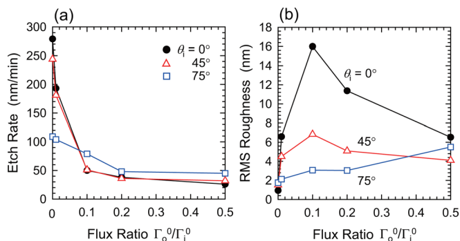
FIG. 10. (Color online) (a) Etch rate and (b) rms surface roughness at t=60 s as a function of oxygen-to-ion flux ratio in the range \Gamma_o^0/\Gamma_i^0 = 0-0.5 with ion incidence angles of \theta_i = 0^\circ, 45^\circ , and 75^\circ derived from the simulations of Fig. 9.
