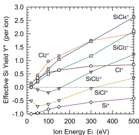
FIG. 21. (Color online) Effective Si yield Y^* per ion impact as a function of incident energy E_i , obtained through the MD simulation of \text{Cl}_x^+ ( x = 1, 2 ) and \text{SiCl}_x^+ ( x = 0 –4) ion incidences on Si(100) surfaces with different E_i = 20 –500 eV at \theta_i = 0^\circ (normal incidence) as shown in Fig. 20. [Reproduced in part with permission from N. Nakazaki, Y. Takao, K. Eriguchi, and K. Ono, Jpn. J. Appl. Phys. 53 , 056201 (2014). Copyright 2014 The Japan Society of Applied Physics.] Note that in the case of \text{Cl}_x^+ incidence, the effective Si yield Y^* (per ion) equals the Si yield Y (per ion), which is defined as the total number of Si atoms desorbed from substrate surfaces per ion impact; on the other hand, the effective yield is Y^* = Y - 1 in the case of \text{SiCl}_x^+ incidence, because one Si atom is incident on surfaces per \text{SiCl}_x^+ impact. Thus, the positive Y^* indicates the etching, while the negative Y^* indicates the deposition.
