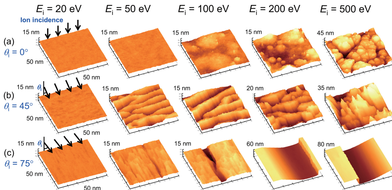
Fig. 5. (Color online) Surface features of Si at t = 60 s after the start of etching in \text{Cl}_2 plasma, simulated for different ion energies in the range E_i = 20 –500 eV with ion incidence angles of \theta_i = (a) 0^\circ , (b) 45^\circ , and (c) 75^\circ . The other calculation conditions in the ASCeM-3D are the same as those of Fig. 3 ( \Gamma_n^0/\Gamma_i^0 = 100 , \Gamma_o^0 = \Gamma_p^0 = 0 ). Note that the surface features for E_i = 100 eV of interest here are the same as those shown at t = 60 s in Figs. 3(a), 3(d), and 3(f).
