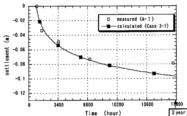
Fig. 16 Settlement comparing between measured and calculated(case3) values
