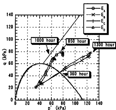
Fig. 10 Effective stress pass (Reinforced by GHD-case2)
