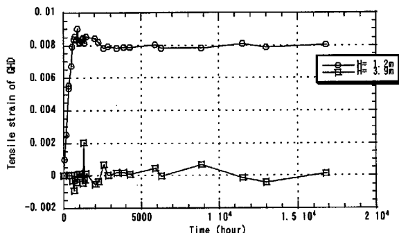
Fig. 6 Tensile strain of GHD
