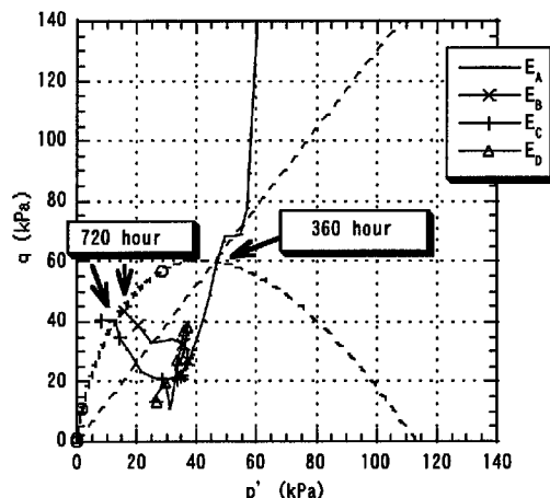
Fig. 8 Effective stress pass (No reinforcement by GHD)
