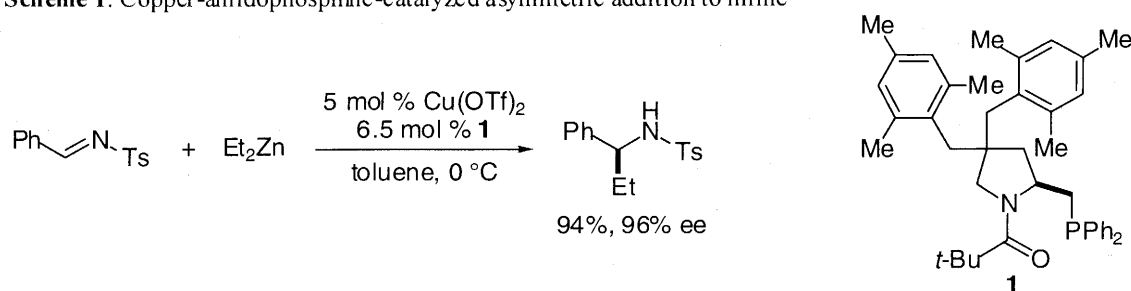
Scheme 1. Copper-amidophosphine-catalyzed asymmetric addition to imine
