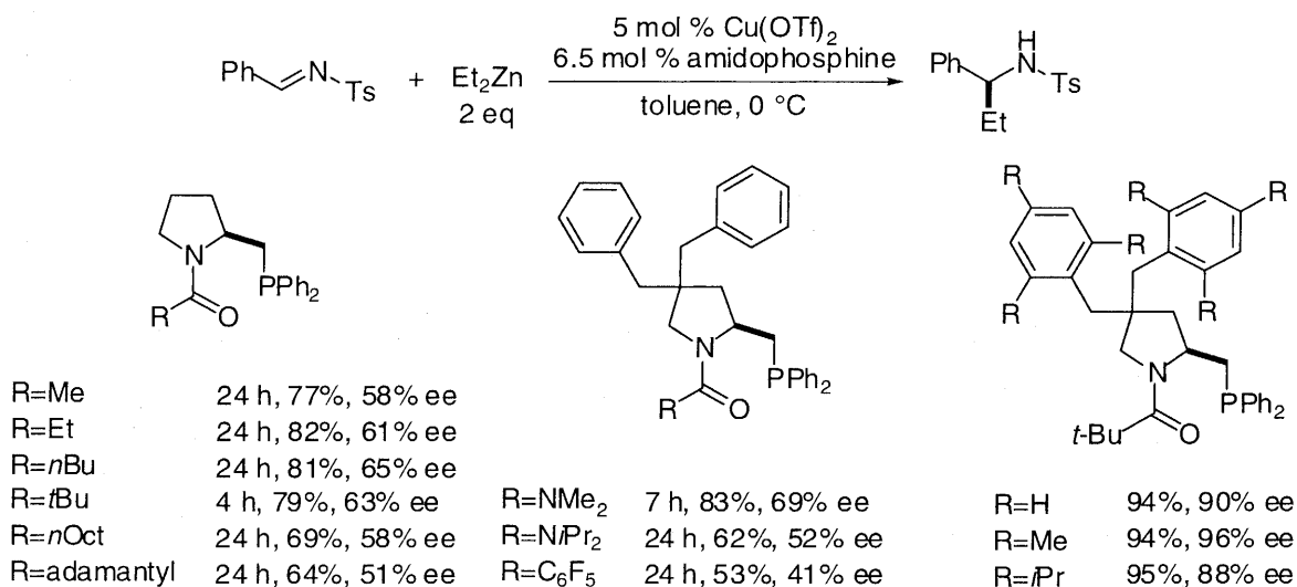
Scheme 3. Effects of amidophosphines
