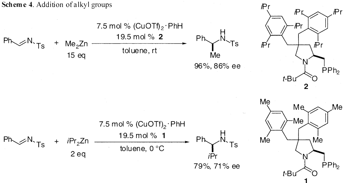
Scheme 4. Addition of alkyl groups
