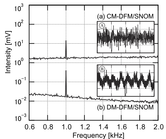
FIG. 3. Frequency spectra and signal waveforms of input signal to lock-in amplifier. (a) CM method. (b) DM method.
