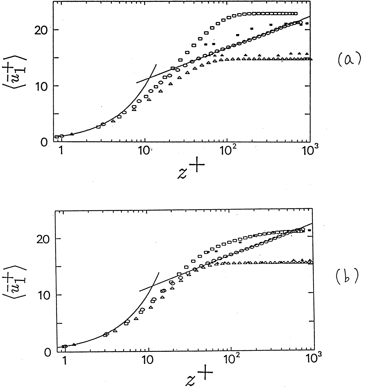
FIG. 3. Mean streamwise velocity profiles \langle \bar{u}_1^+ \rangle : \bigcirc , H_a = 0 ; \square , H_a = 52.5 ; \triangle , H_a = 125 ; \blacksquare , experimental data of Brouillette and Lykoudis at H_a = 52.5 ; \blacktriangle , experimental data of Brouillette and Lykoudis at H_a = 125 ; —, \langle \bar{u}_1^+ \rangle = z^+ ( z^+ \leq 10 ) and \langle \bar{u}_1^+ \rangle = (1/0.41) \ln z^+ + 5.5 ( z^+ \geq 10 ).
