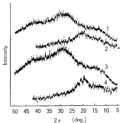
Fig. 13 X-ray diffraction curves of regenerated holo- and \alpha -celluloses precipitated from its \text{SO}_2 -DEA-DMSO sol. with water or chloroform. 1: holocellulose, regenerated by water; 2: holocellulose, by \text{CHCl}_3 ; 3: \alpha -cellulose, by water; 4: \alpha -cellulose, by \text{CHCl}_3 .
