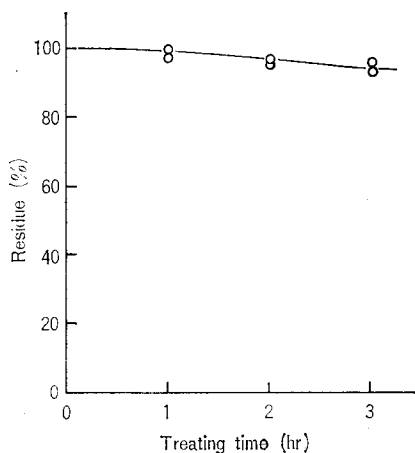
Fig. 7 Relation between unsolved residue of wood treated with \text{SO}_2 -diethylamine (DEA)-DMSO solution and treating time. ( \text{SO}_2 5%, \text{SO}_2 : DEA = 1:1 moles, wood: solution = 1:10 by weight, 140^\circ\text{C} )
