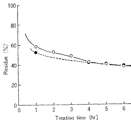
Fig. 1 Decrease in unsolved wood residues with treating time for solution of 5% \text{SO}_2 in DMSO at 140^\circ\text{C} . ○: no water, ●: 5% water added
