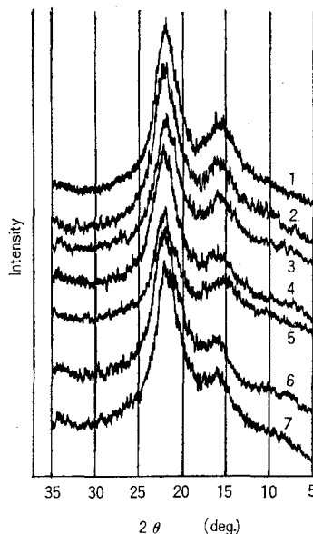
Fig. 11 X-ray diffraction curves of wood treated with DEA or DEA-DMSO sol. 1 : DEA, 140^\circ\text{C} , 3hr; 2 : 70% DEA-DMSO, 140^\circ\text{C} , 3hr; 3 : 60% DEA-DMSO, 140^\circ\text{C} , 3hr; 4 : 10% DEA-DMSO, 140^\circ\text{C} , 3hr; 5 : DEA, 20^\circ\text{C} , 24hr; 6 : 80% DEA-DMSO, 20^\circ\text{C} , 24hr; 7 : 20% DEA-DMSO, 20^\circ\text{C} , 24hr.
