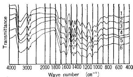
Fig. 3 Infrared spectra of precipitates prepared from cooking liquors by addition of water. Cooking conditions are as follows : 1 : 5 % SO 2 -DMSO, 140°C, 1hr ; 2 : 10% SO 2 , 140°C, 1hr ; 3 : 10% SO 2 , 140°C, 2hr ; 4 : 5% SO 2 -5% H 2 O-, 140°C, 3hr ; 5 : 10% SO 2 , 140°C, 3hr ; 6 : 5 % SO 2 , 140°C, 6hr.
