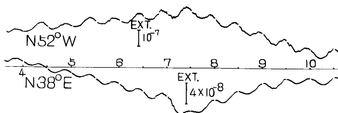
Fig. 13 (B) Records of extensometers
