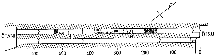
Fig. 2 Location of instruments
