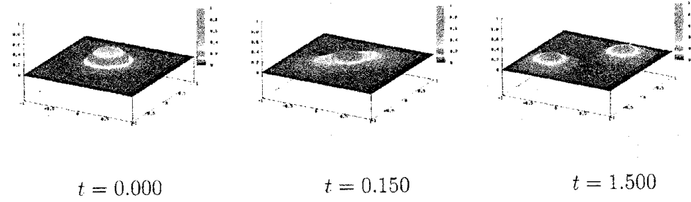
Figure 4: The bubble is divided to two by the non-uniform distribution of Q^2 .
