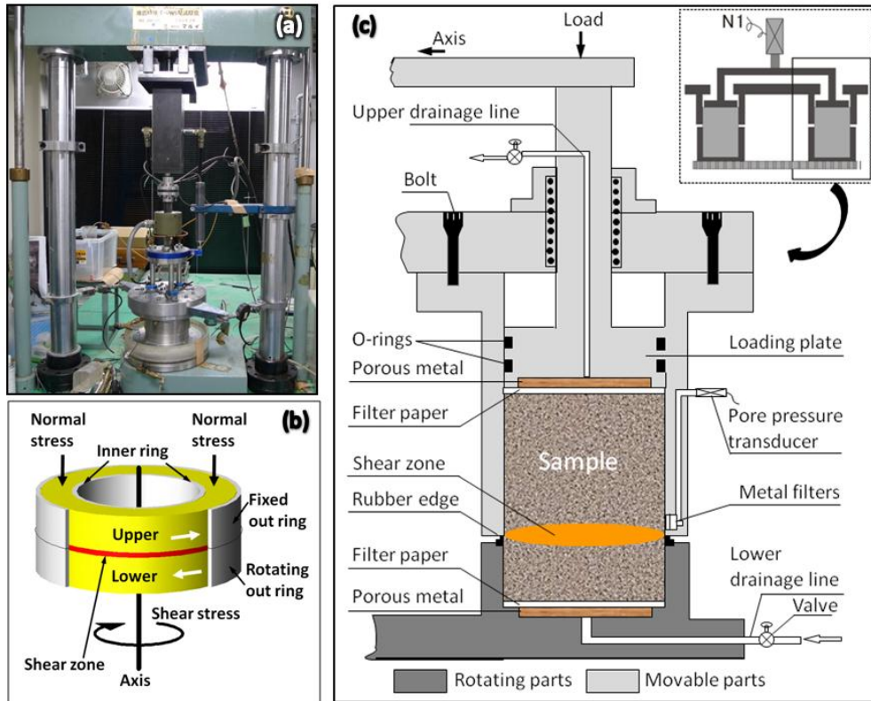
Fig. 5. Ring-shear apparatus DPRI-Ver.5. (a) Overview; (b) sample in ring-shear box; (c) half of the cross section through center of undrained shear box
