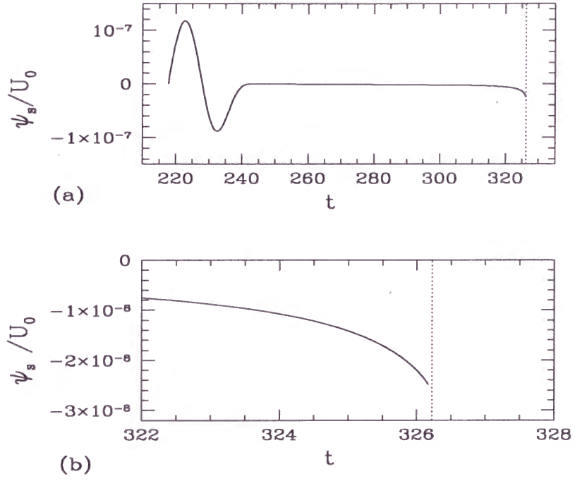
Figure 6.9: \psi_s for globally-naked-singular space-time at R = 100M . In (a) the initial oscillation is due to the choice of initial data. (b) is the magnification of (a). The dotted line denotes the Cauchy horizon.
