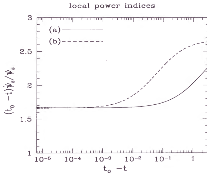
Figure 6.8: Local power index \delta^{\text{local}} . The solid and broken lines denote (a) the globally-naked singular and (b) the locally-naked-singular space-times, respectively.
