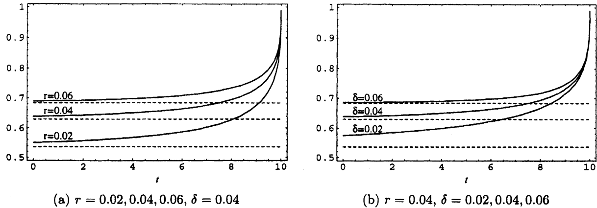
Figure 1: Early exercise boundaries \underline{S}(m, T - t)/m ( T = 10, \sigma = 0.2 )
