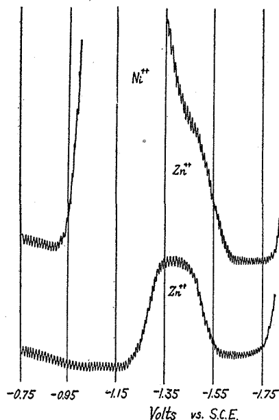
Fig. 5. Differential polarogram of zinc ( \Delta E=200\text{mV} ).
