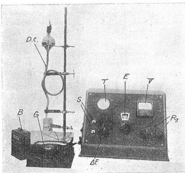
Fig. 1. Concentration-meter.
