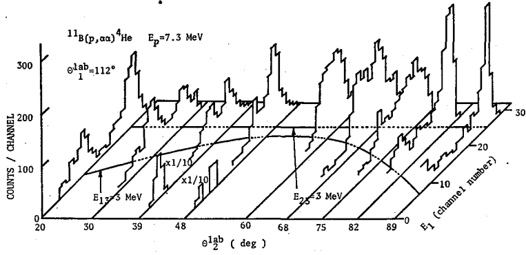
Fig. 7. Plot of coincidence energy spectra against \theta_2^{\text{lab}} for \theta_1^{\text{lab}} = 112^\circ . The straight and curved lines represent the calculated loci corresponding E_{23} = 3.0 MeV and E_{13} = 3.0 MeV, respectively.
