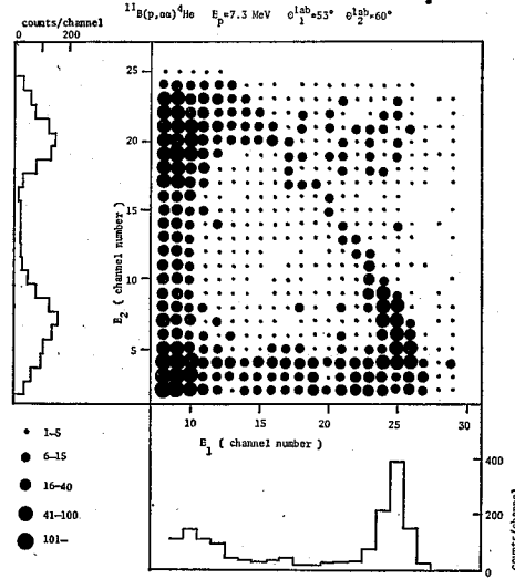
Fig. 5. Coincidence energy spectrum of alpha particles from the ^{11}\text{B}+p \rightarrow 3\alpha reaction. Histograms below and left represent the energy spectra projected onto the E_1 and E_2 axes.
