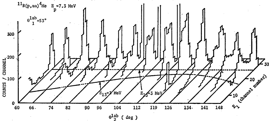
Fig. 6. Plot of coincidence energy spectra against \theta_2^{\text{lab}} for \theta_1^{\text{lab}}=53^\circ . The straight and curved lines represent the calculated loci corresponding E_{23}=3.0 MeV and E_{13}=3.0 MeV, respectively.
