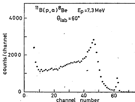
Fig. 1. Energy spectrum of alpha particles from the ^{11}\text{B}(p, \alpha)^8\text{Be} reaction.
