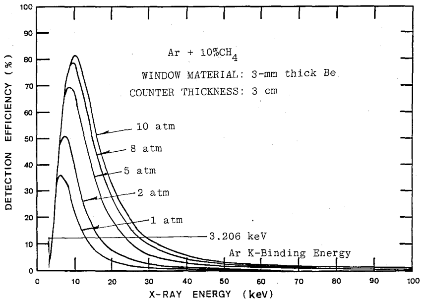
Fig. 4. Detection efficiency of Ar + 10%CH 4 as a function of the gas pressure; the window material is 3-mm thick beryllium and the counter thickness is 3 cm.
