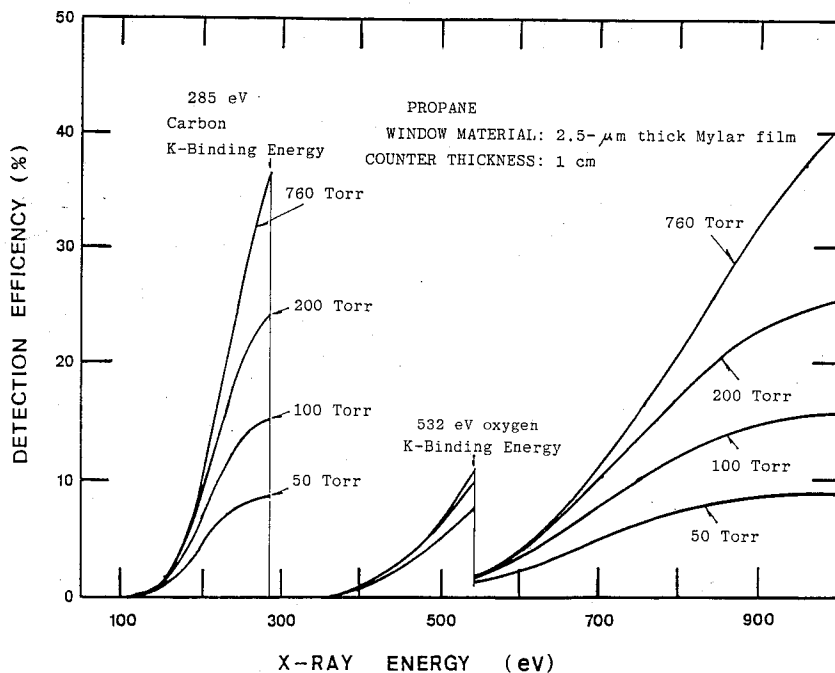
Fig. 3. Detection efficiency of propane ( \text{C}_3\text{H}_8 ) as a function of the gas pressure; the window material is 2.5- \mu\text{m} thick Mylar film and the counter thickness is 1 cm.
