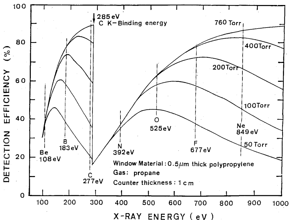
Fig. 1. Detection efficiency of propane ( C_3H_8 ) as a function of the gas pressure; the window material is 0.5- \mu m thick polypropylene and the counter thickness is 1 cm.
