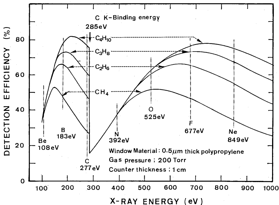
Fig. 2. Detection efficiencies of methane ( \text{CH}_4 ), ethane ( \text{C}_2\text{H}_6 ), propane ( \text{C}_3\text{H}_8 ) and isobutane ( \text{C}_4\text{H}_{10} ) at a gas pressure of 200 Torr; the window material is 0.5\text{-}\mu\text{m} thick polypropylene and the counter thickness is 1 cm.
