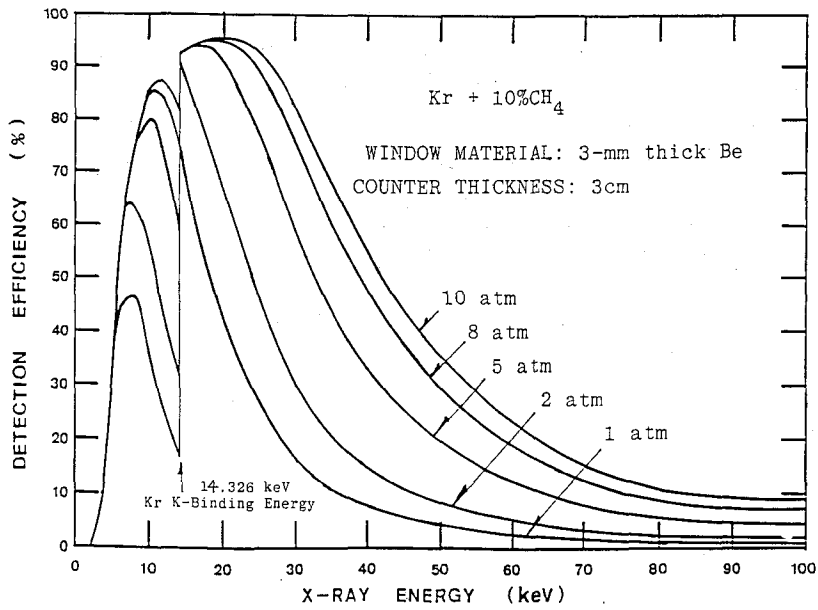
Fig. 5. Detection efficiency of Kr + 10%CH 4 as a function of the gas pressure; the window material is 3-mm thick beryllium and the counter thickness is 3 cm.
