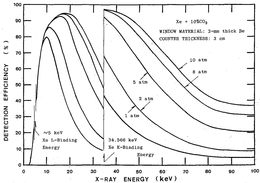
Fig. 6. Detection efficiency of Xe + 10%CO 2 as a function of the gas pressure; the window material is 3-mm thick beryllium and the counter thickness is 3 cm.
