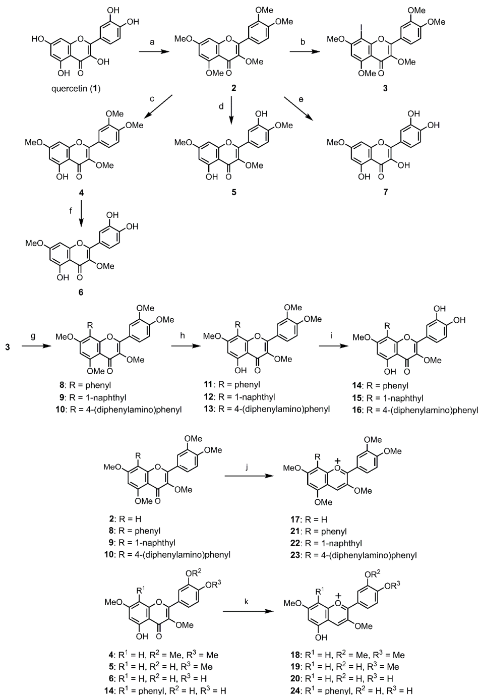
Scheme 1. Synthetic plan of O-methylquercetins (2–16) and O-methylanthocyanidins (17–23). (a) MeI (29 eq.), NaH (7.6 eq.), DMF, 80 °C; (b) NIS (1.2 eq.), DMF, 70 °C; (c) BBr 3 (2.0 eq.), MeCN, rt; (d) BBr 3 (2.0 eq.), CH 2 Cl 2 , −30 °C; (e) BBr 3 (3.0 eq.), CH 2 Cl 2 , 0 °C; (f) BCl 3 (5.3 eq.), TBAI (5.3 eq.), CH 2 Cl 2 , −20 °C; (g) 8: phenylboronic acid (2.0 eq.), Pd(OAc) 2 (3.0 mol %), K 3 PO 4 (3.0 eq.), toluene, 100 °C; 9: 1-naphthaleneboronic acid (2.0 eq.), Pd(OAc) 2 (3.0 mol %), K 3 PO 4 (3.0 eq.), PPh 3 (3.0 mol %), CPME, 100 °C; 10: 4-(diphenylamino)phenylboronic acid (1.5 eq.), Pd(OAc) 2 (1.5 mol %), K 2 CO 3 (2.0 eq.), EtOH/H 2 O, 80 °C; (h) BBr 3 (3.0 eq.), CPME, 0 °C → rt; (i) BCl 3 (5.3 eq.), TBAI (5.3 eq.), CH 2 Cl 2 , −20 °C; (j) LiAlH 4 (4.0 eq.), THF, rt; (k) Zn, HCl-MeOH, 0 °C and then air, HCl-MeOH, rt.
