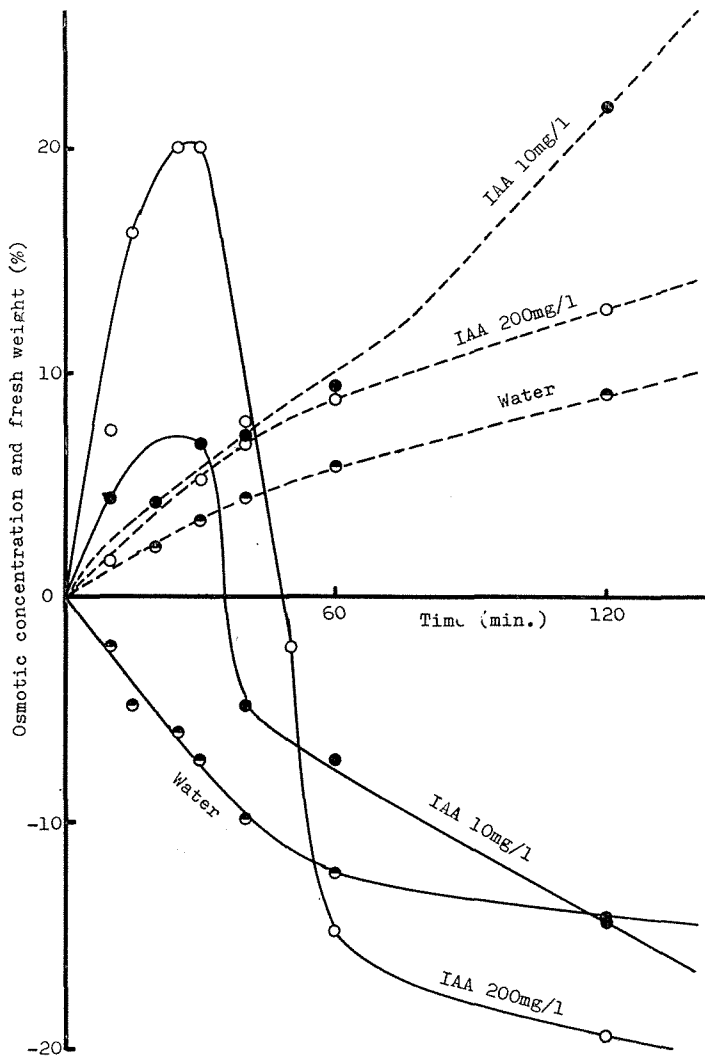
Fig. 2. Effect of IAA on the osmotic value (—) and water absorption (---) of pea stem sections floated on IAA solutions and water. The values after the various periods of treatment are expressed in percentage of the values at 0 time.
