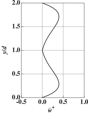
Figure 2: Profile of spanwise base flow \bar{w}^+ .
