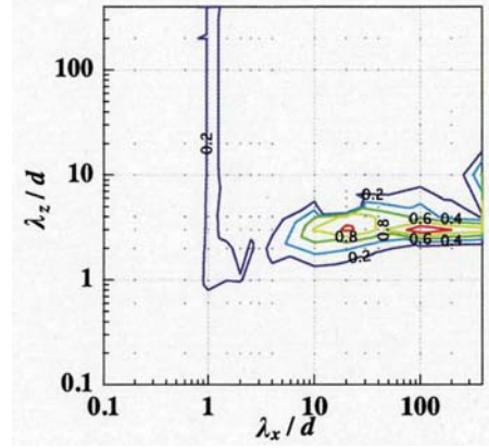
Figure 3: Contour of increase of the global amplification rates with spanwise base flow for each wavelength modes, G_{global,diff} .
