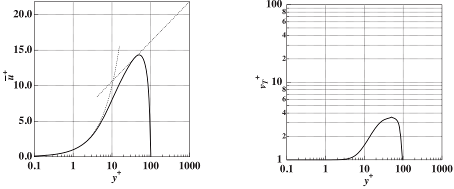
Figure 1: Profiles of streamwise base flow \bar{u}^+ (left), and the total eddy viscosity \nu_T^+ (right).
