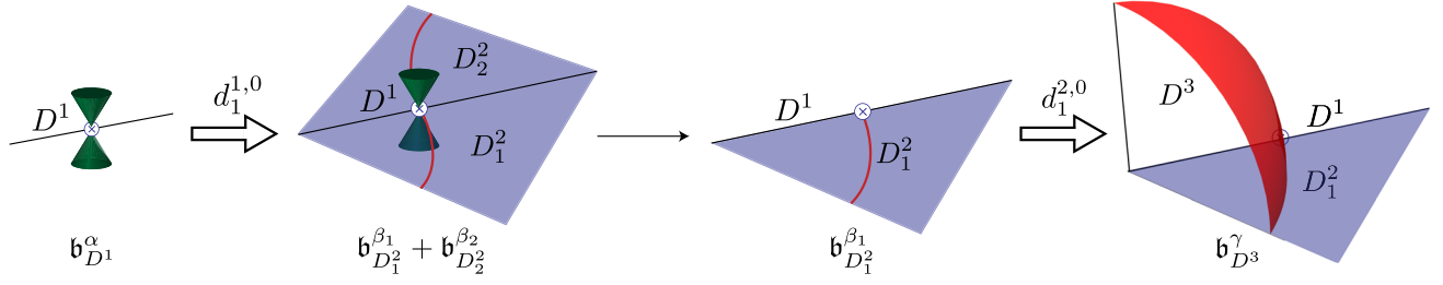
FIG. 12. Illustration of the diagnostic scheme for case A. We begin by acting d_1^{1,0} on a generator of E_1^{1,0} corresponding to a basis \mathbf{b}_{D^1}^\alpha . Then, we obtain the gapless lines on the 2-cells adjacent to the 1-cell D^1 , which is an element of E_1^{2,0} . Next, we focus on one of the adjacent 2-cells. In the figure, we pick D_1^2 from the two 2-cells. In other words, we consider only \mathbf{b}_{D_1^2}^{\beta_1} of \mathbf{b}_{D_1^2}^{\beta_1} + \mathbf{b}_{D_2^2}^{\beta_2} in the figure. Finally, we map \mathbf{b}_{D_1^2}^{\beta_1} to an element E_1^{3,0} by d_1^{2,0} and examine whether the mapped element is trivial or not.
