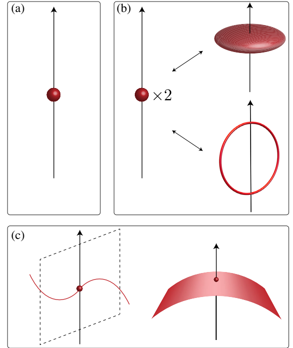
FIG. 3. Illustration of results of gapless point classifications on a line: (a) The gapless point on the line is a genuine point node. (b) A point node formed by multiple gapless points can be realized, but such a point node is actually a shrunk loop or surface node. Since there are no reasons why two gapless points are at the same position, it is natural to consider that a shrunk loop or surface node exists in such a case. (c) The gapless point must be part of a line or surface node.
