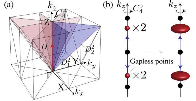
FIG. 15. (a) A half BZ in MSG P4 . Here, the blue planes D_1^2 and D_2^2 are adjacent 2-cells to D^1 , and red ones are symmetry related to D_1^1 and D_2^1 . (b) Deformation of nodal structures in MSG P4 .
