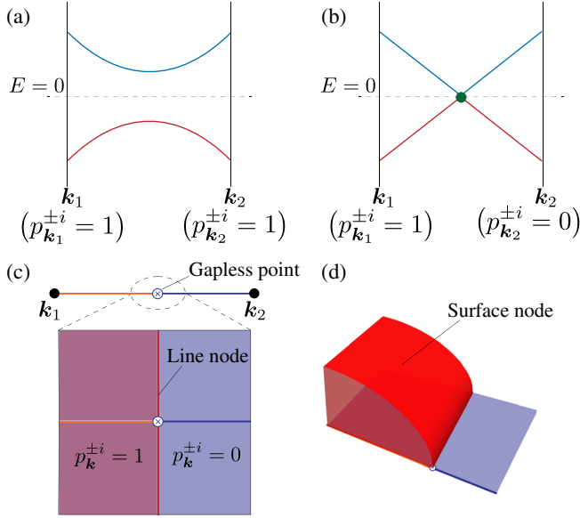
FIG. 2. Illustration of diagnosis based on compatibility conditions. (a),(b) Bogoliubov quasiparticle spectrum along the line connecting two momenta k_1 and k_2 . The spectrum satisfies the compatibility conditions on the line in (a), while it does not in (b). (c) Two divisions of the line connecting k_1 and k_2 and a nodal line in a plane containing the line. Here, the red shaded region and others have different values of the topological invariants, whose boundary results in a nodal line. (d) Surface node. When there are compatibility conditions between the plane and its three-dimensional neighborhood, the regions in (c) are extended out of the plane, and the boundary surface is the surface node.
