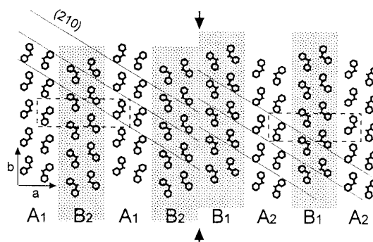
Figure 1. Definition of two types of motifs (1, 3).
