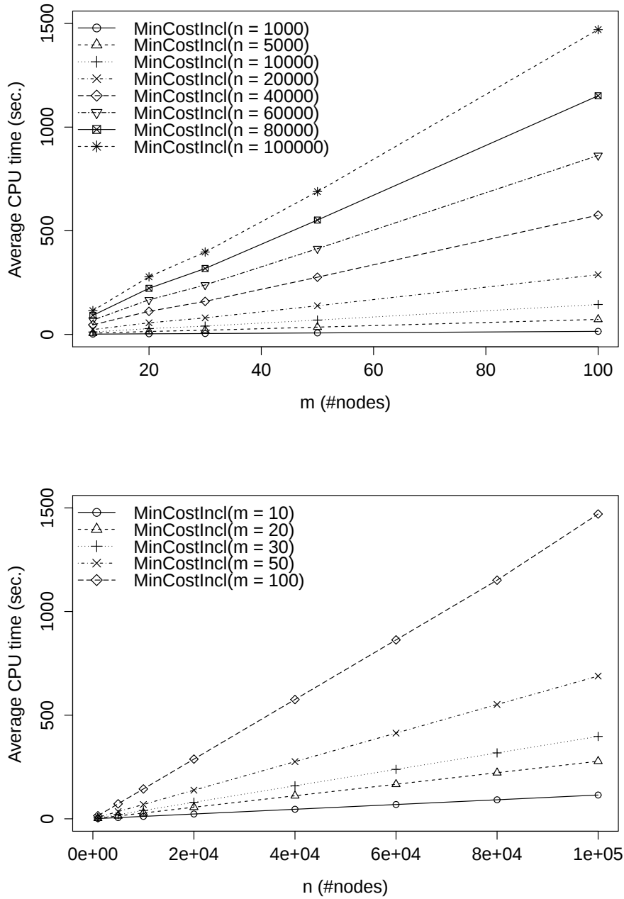
Figure 4.8: Execution times of MinCostIncl for varying sizes of pattern trees (top) and text trees (bottom). Note that m \leq n must hold from the definition of MinCostIncl.
