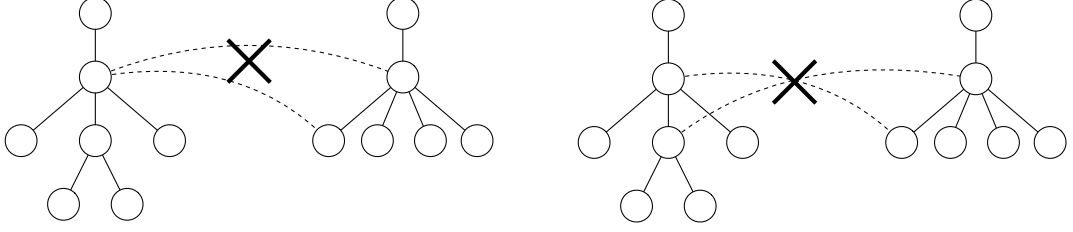
Figure 2.3: Example of the condition of the edit distance mapping. The left and right figures correspond to conditions (i) and (ii) for the edit distance mapping, respectively, where (i) stands for one-to-one condition, and (ii) stands for descendant condition.
