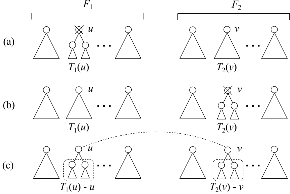
Figure 2.5: Dynamic programming procedure for the edit distance between unordered trees. (a), (b), and (c) denote the top, middle, and bottom of Eq. (2.3), respectively.
