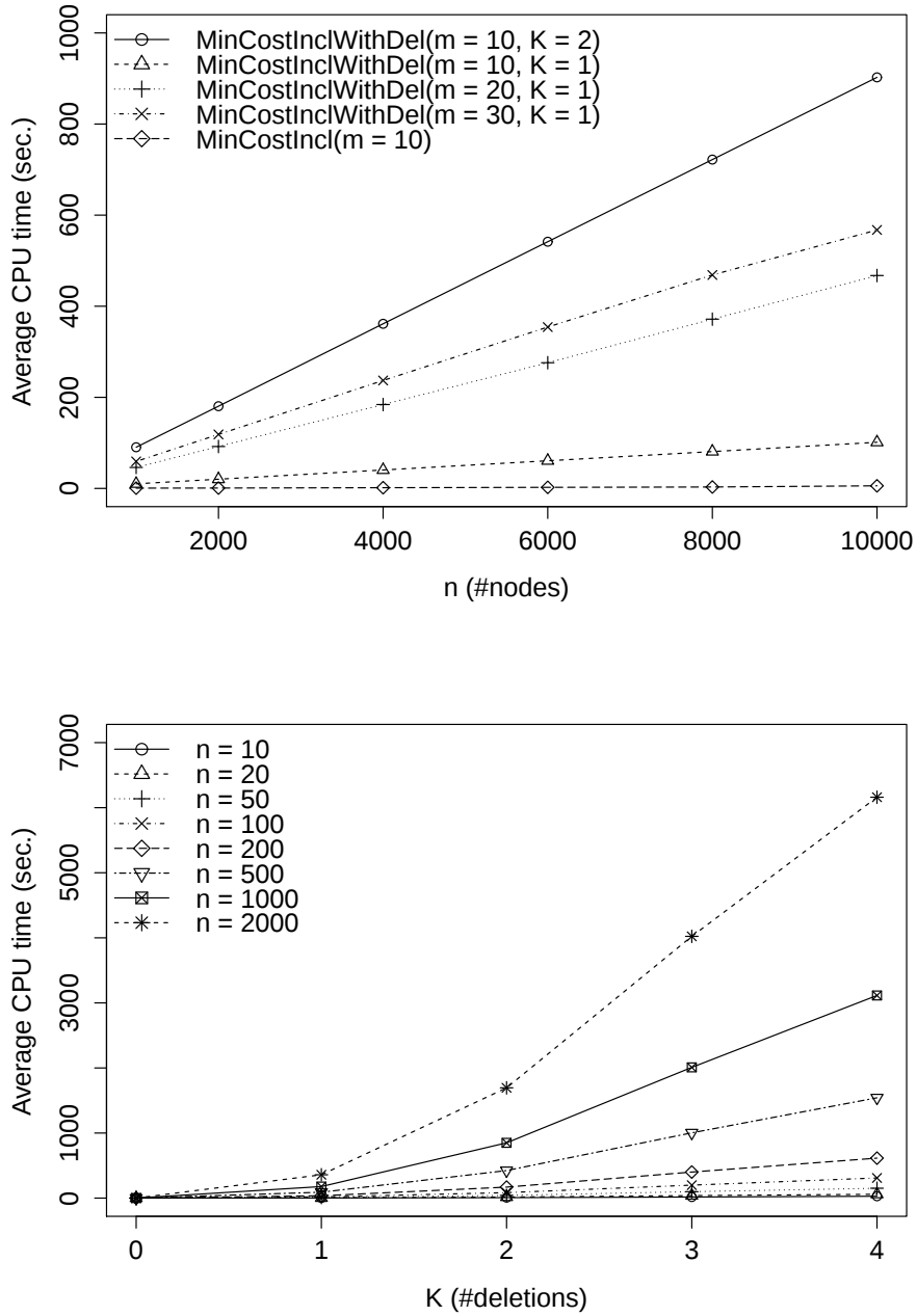
Figure 4.11: Execution times for MinCostInclWithDel with varying n (top) and varying K with m = 10 (bottom).
