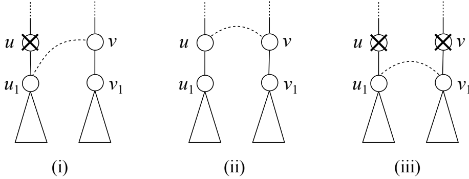
Figure 3.5: Heuristic technique (1). (i), (ii), and (iii) denote the case (i) \sim (iii) in the proof of the Proposition 3.2.2.
