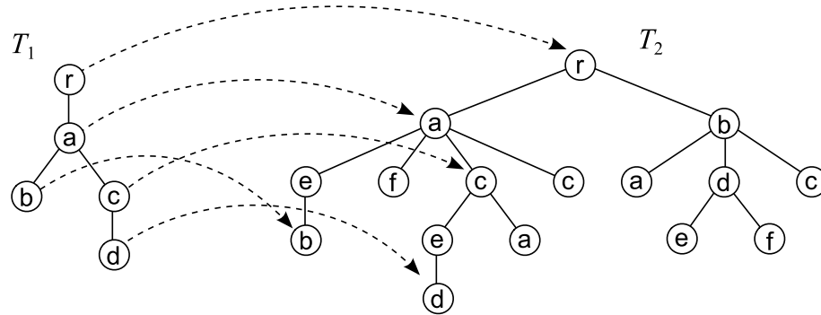
Figure 2.12: Tree inclusion. T_1 is included in T_2 . The embedding between T_1 and T_2 is indicated by dashed curves.
