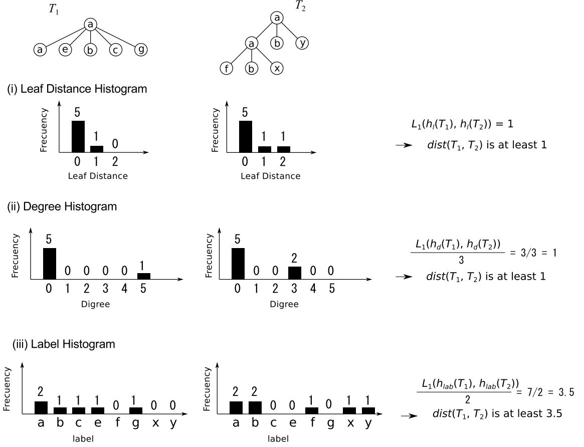
Figure 2.9: Histogram-based estimations for a lower bound of the tree edit distance. T_1 and T_2 are input trees. (i), (ii), and (iii) represent the leaf distance histogram, the degree histogram, and the label histogram of the input trees, respectively.
