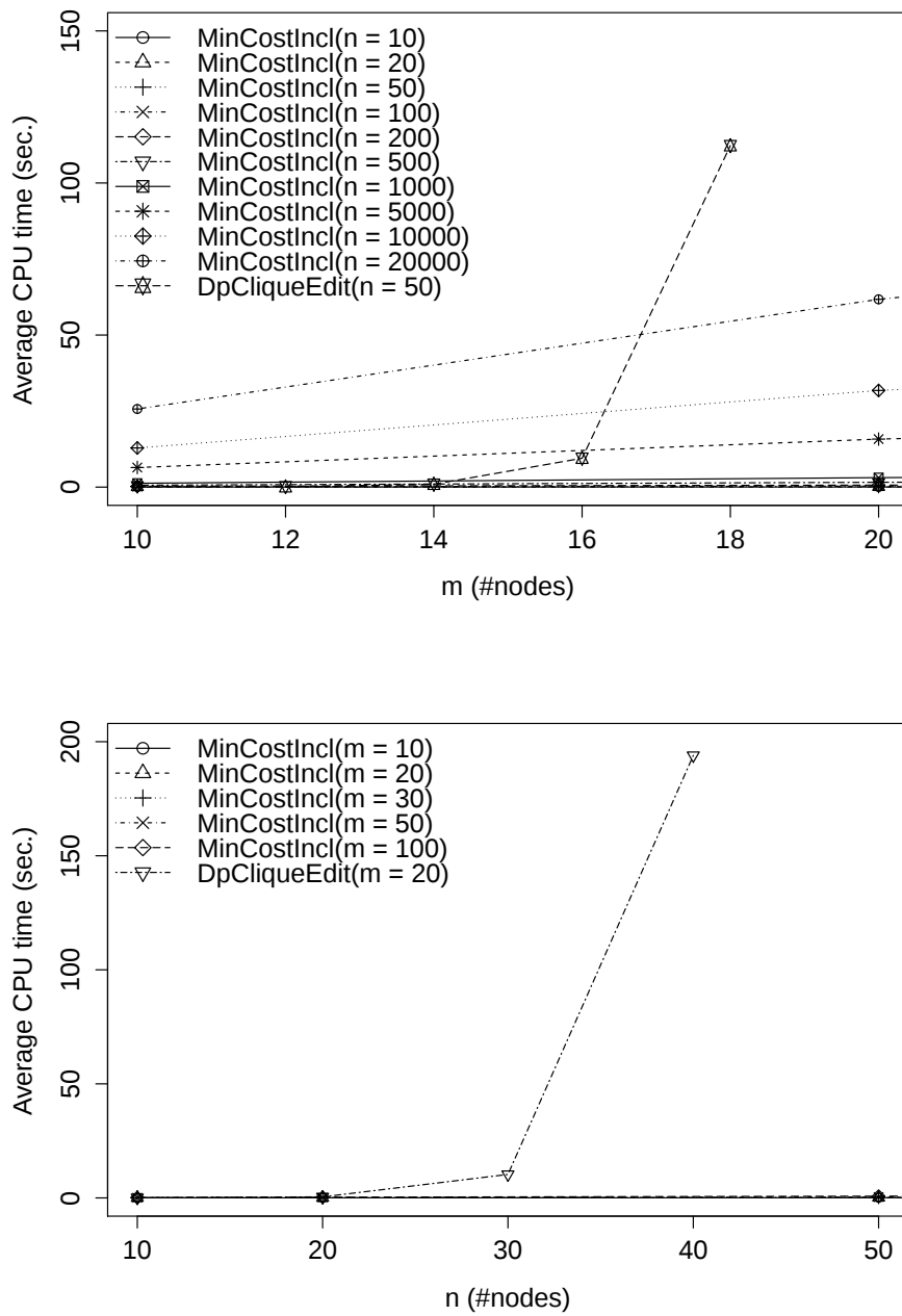
Figure 4.9: Comparison between MinCostIncl and DpCliqueEdit for varying sizes of pattern trees (top) and text trees (bottom).
