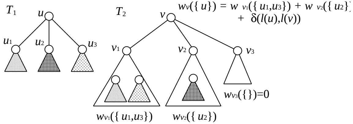
Figure 4.4: Illustrating the computation of minimum-cost tree inclusion. Here, u is mapped to v .
