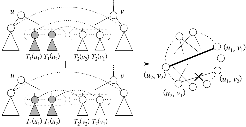
Figure 3.8: Example of heuristic technique (5). T_1(u_1) and T_1(u_2) are isomorphic including label information. In this case, we need not create \{(u_1, v_2), (u_2, v_1)\} .
