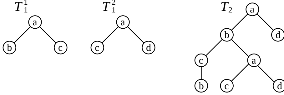
Figure 4.2: Both T_1^1 and T_1^2 are included in T_2 . However, T_1^2 looks like a more similar subtree since it is isomorphic to a rooted subtree of T_2 .
