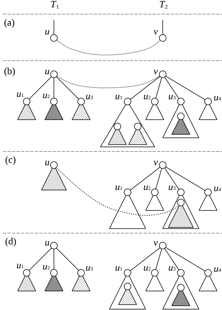
Figure 4.5: The four cases in the proof of Theorem 4.3.2.
