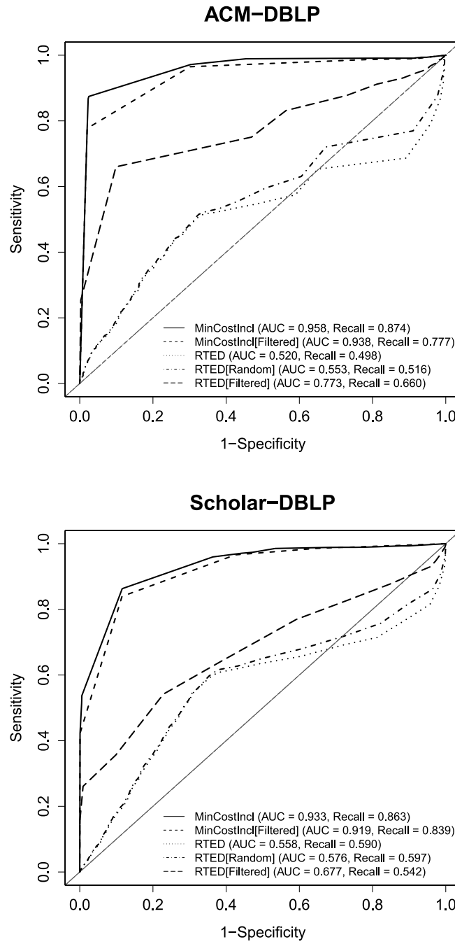
Figure 4.14: Comparison of accuracy for ACM-DBLP data (top) and Scholar-DBLP data (bottom).
