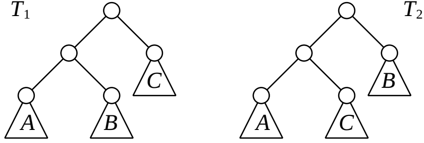
Figure 2.4: Comparing the ordered and unordered tree edit distance. The ordered tree edit distance is 2x while the unordered tree edit distance is 2.
