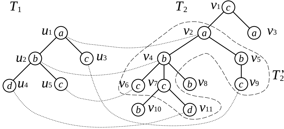
Figure 4.1: An example of unordered tree inclusion.
