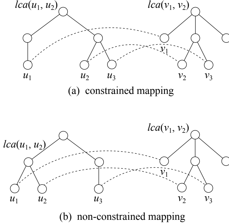
Figure 2.7: Example of constrained mapping.
