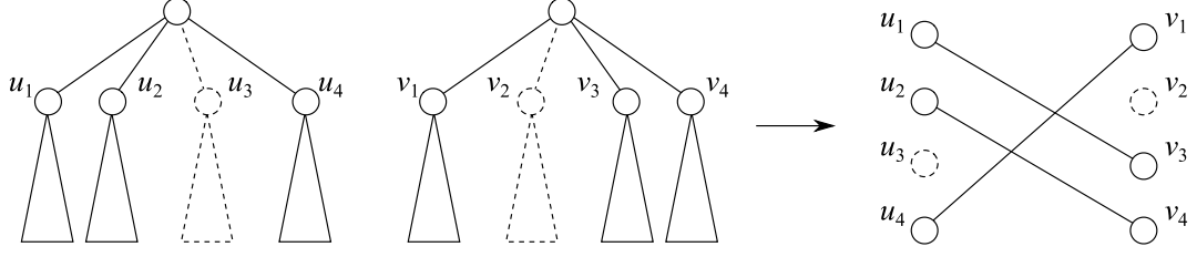
Figure 2.6: Example of the fixed-parameter algorithm. T_1(u_3) and T_2(v_2) are deleted when they are isomorphic, and then the residual subtrees are matched.
