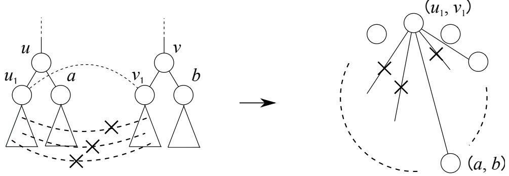
Figure 3.4: Difference between the reductions in CliqueEdit and DpCliqueEdit. In computation of W[u, v] in DpCliqueEdit, vertex (u_1, v_1) in G_{(u,v)} is not connected to any one of vertices corresponding to pairs of descendants of u_1 and v_1 .
