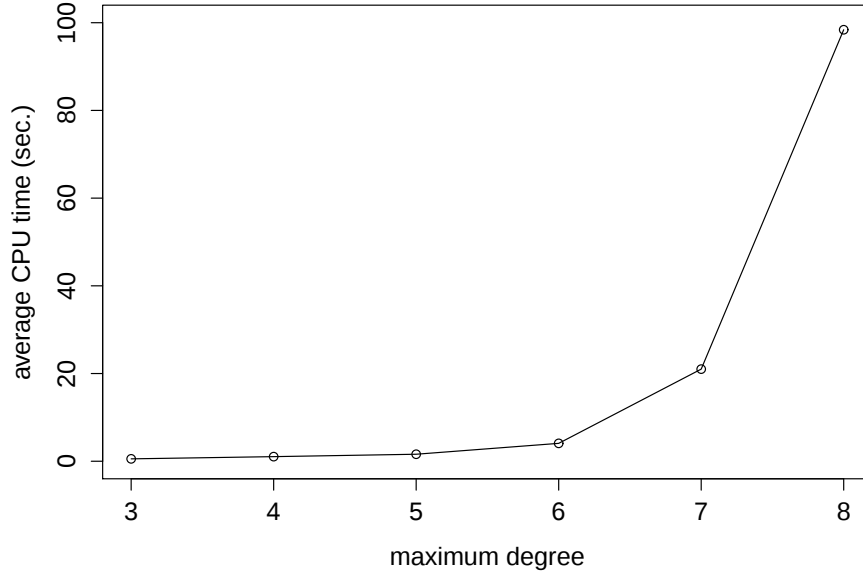
Figure 4.12: Execution times for weblogs data.
