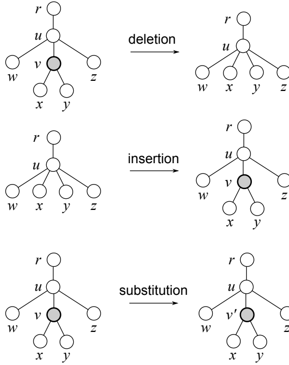
Figure 2.1: Edit operations on a tree. The top, middle, and bottom indicate a deletion, an insertion, and a substitution operation, respectively.
