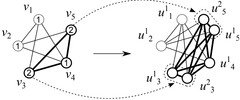
Figure 3.3: Example of transformation of a vertex weighted graph into an unweighted graph. v_3 and v_5 are duplicated.
