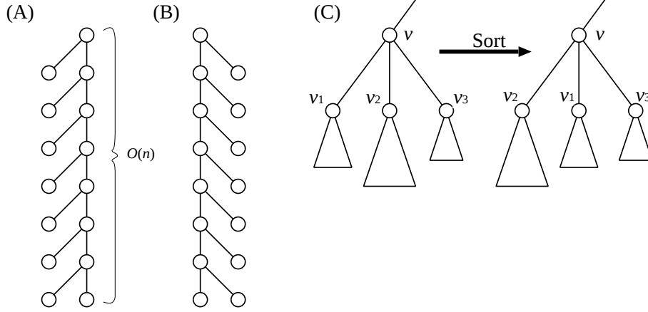
Figure 4.6: Improving the space complexity. (A) needs O(n + 2^D mn) space, whereas (B) needs O(n + 2^D m) space. To minimize the space, it is enough to sort the children as in (C).
