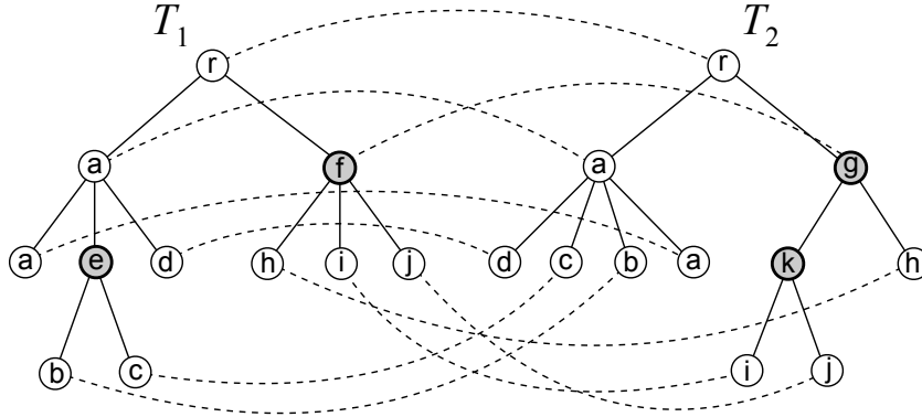
Figure 2.2: Example of tree edit operations and edit distance mapping for unordered trees. T_2 is obtained from T_1 by deletion of node labeled e , insertion of node labeled k , and substitution of node labeled f with node labeled g , where a tree can contain nodes with the same label. The corresponding mapping M is shown by broken curves.
