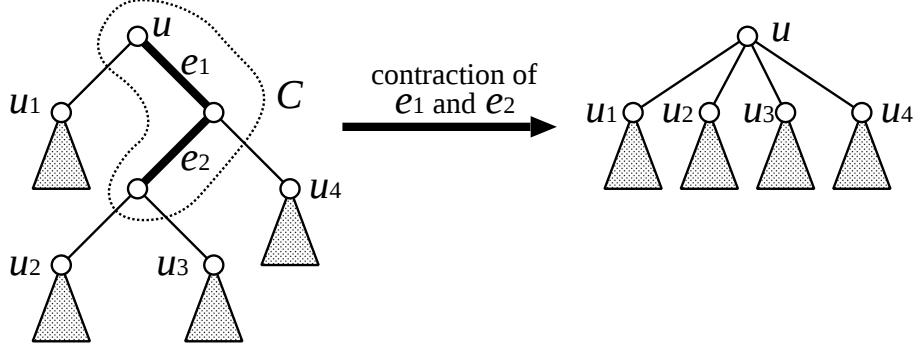
Figure 4.7: A contraction of a connected subtree. In this case, chd(u, C) = \{u_1, u_2, u_3, u_4\} .
