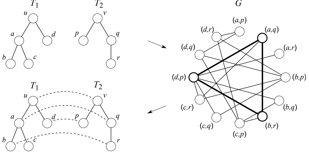
Figure 3.2: Example of a reduction in the previous method (CliqueEdit). A maximum clique is shown by bold lines in graph G , and the corresponding mapping is shown by broken lines in bottom left side.
