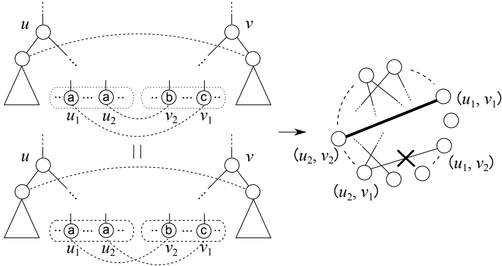
Figure 3.7: Example of heuristic technique (3). u_1, u_2, v_1 , and v_2 are leaves, and \ell(u_1) = \ell(u_2) . In this case, we need not create \{(u_1, v_2), (u_2, v_1)\} .
