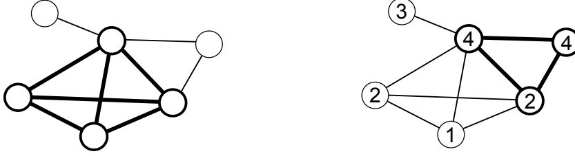
Figure 3.1: Example of the maximum clique and the maximum vertex weighted clique. The size of the maximum clique of the left graph is four, while the weight of the maximum vertex weighted clique of the right graph is 10.
