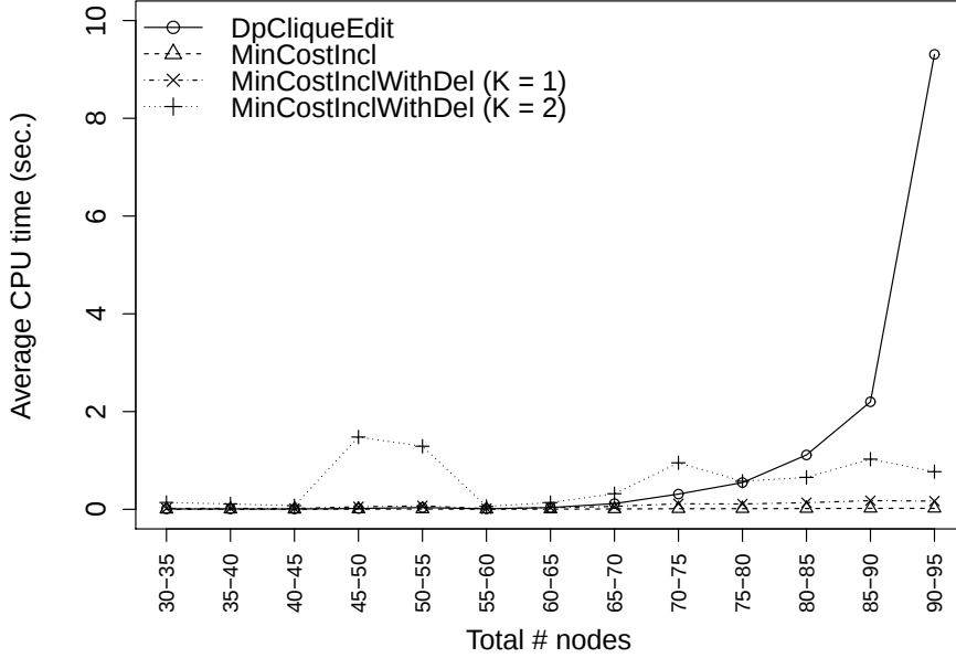
Figure 4.15: Execution times for glycan data.
