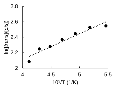
Figure S2. Plots of the cis-trans isomerization ratios toward temperature in DCB-OMe .
