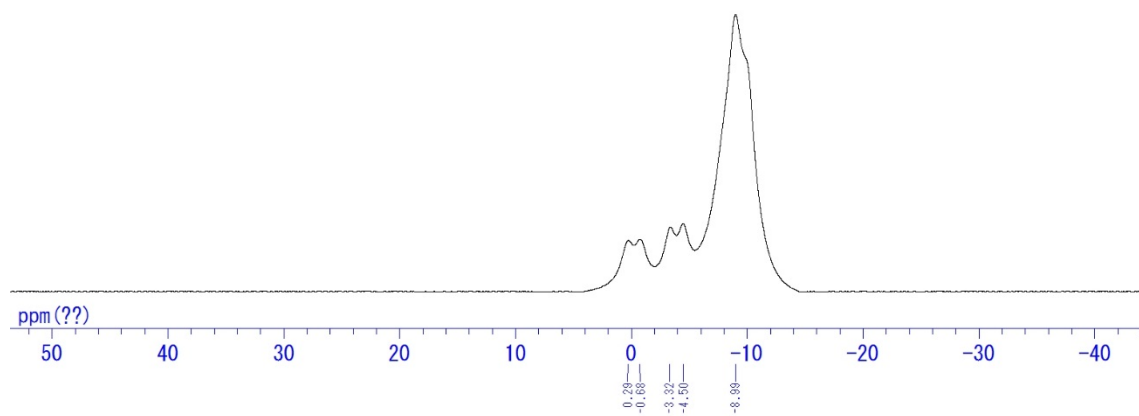
Chart S3. ^{11}\text{B} NMR spectrum of DCB-OMe in \text{CD}_2\text{Cl}_2 .
