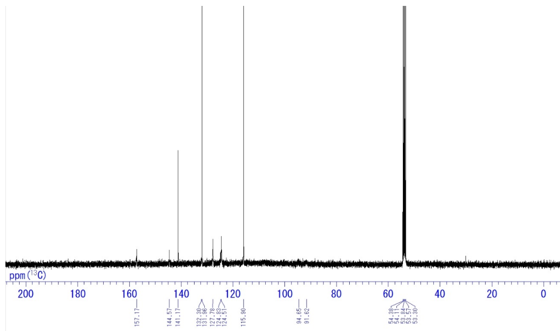
Chart S8. ^{13}\text{C} NMR spectrum of DCB-OH in \text{CD}_2\text{Cl}_2 .
