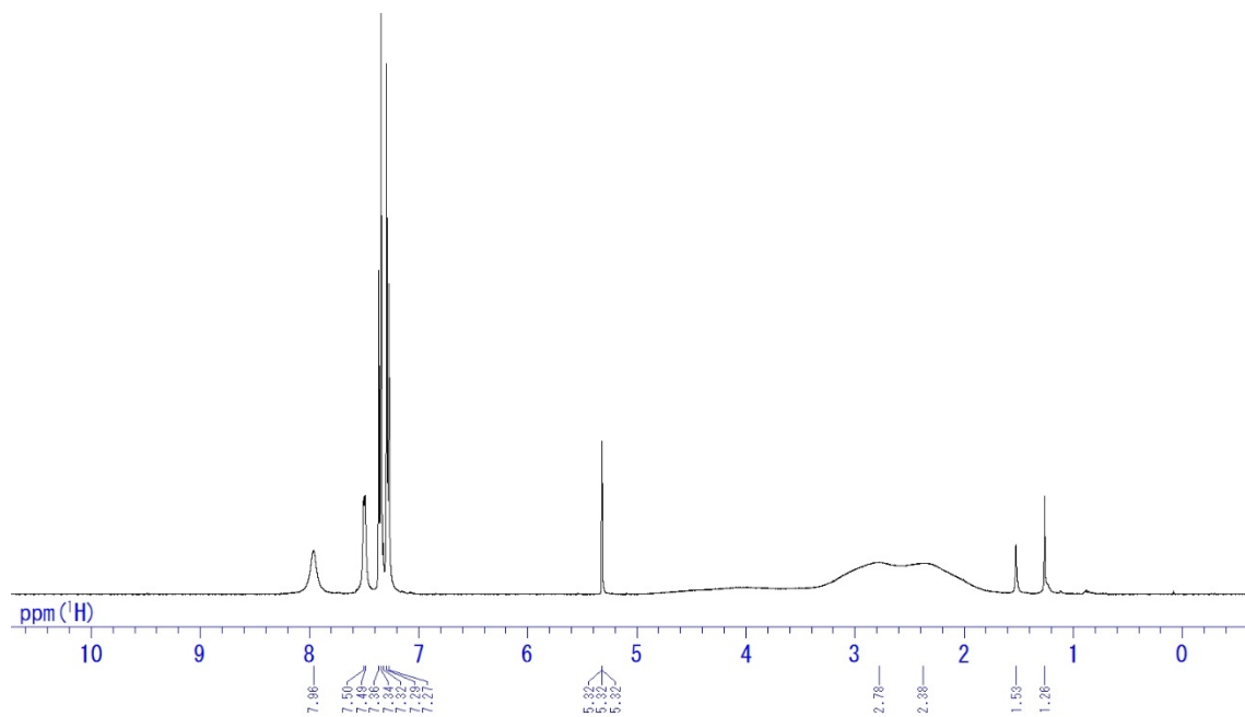
Chart S4. ^1\text{H} NMR spectrum of DCB-CN in \text{CD}_2\text{Cl}_2 .
