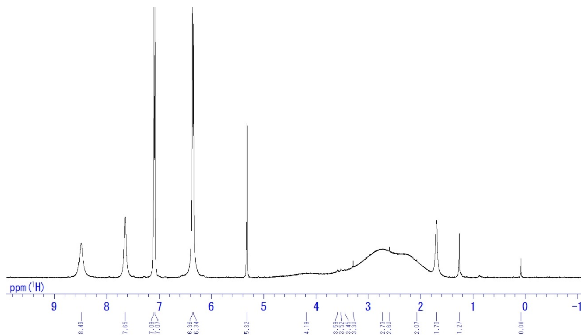
Chart S7. ^1\text{H} NMR spectrum of DCB-OH in \text{CD}_2\text{Cl}_2 .
