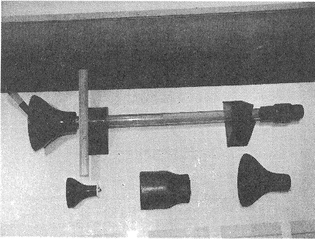
Fig. 3 Reynolds' bellmouth (a).
