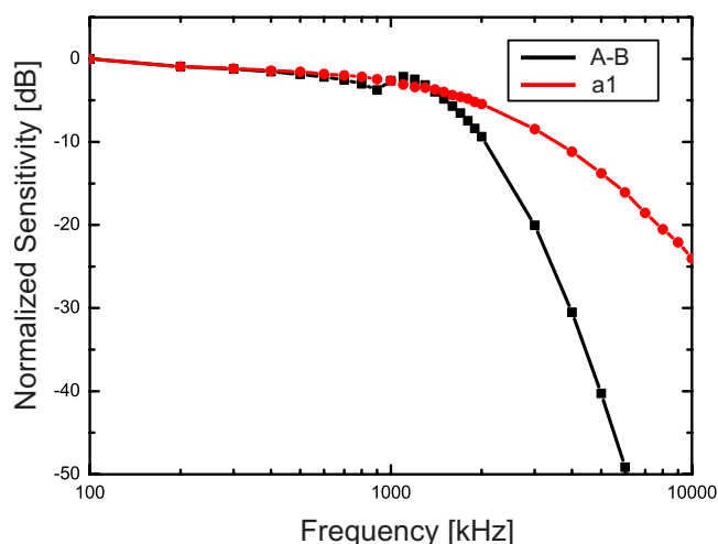
FIG. 1. (Color online) Frequency characteristics of the sensitivity of the OBD sensor: The red curve (a1) shows the normalized sensitivity of the photodiode and the preamplifier. The black curve (A-B) shows the normalized sensitivity of the OBD sensor including the differential amplifier.
