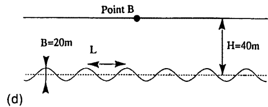
Fig. 15 Effects of the wavelength of irregular boundary on the ground response. (a) L = 320\text{m} . (b) L = 1280\text{m} . (c) L = 2560\text{m} . (d) Boundary shape and location of observation point.
