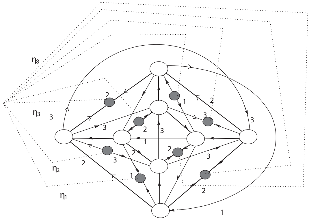
Figure 3.1: Singular chart of Theorem 3.1.
