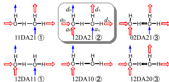
Fig. 1 Examples of the hydrogen-bonding patterns represented by d_b a_D D A d_A a_A . The number in circle corresponds to the M_{OH} value.
