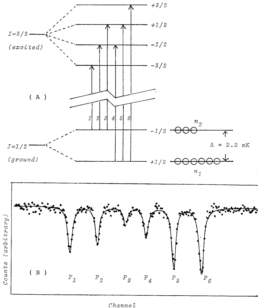
Fig. 3 (A). Nuclear energy scheme for ^{57}\text{Fe} in the presence of a magnetic hyperfine field. \Delta represents the Zeeman splitting of the ground state. n_1 and n_2 are the populations at the levels for -1/2 and +1/2 , respectively.
