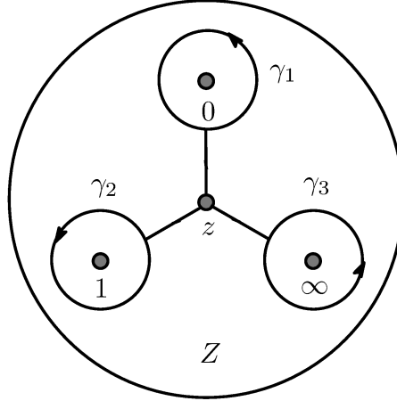
Figure 1. Three basic loops in Z := \mathbb{P}^1 \setminus \{0, 1, \infty\}
