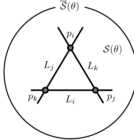
Figure 2. Tritangent lines at infinity on \overline{\mathcal{S}}(\theta)
