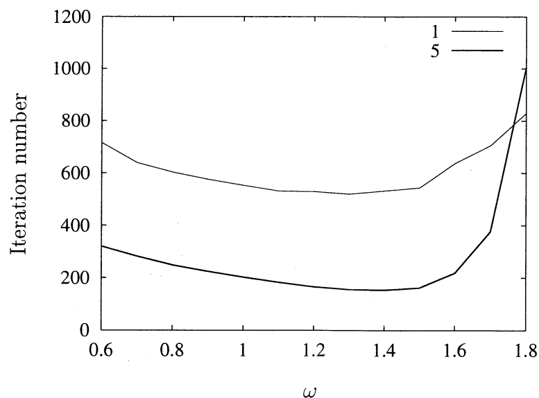
Fig. 4. Iteration numbers to relaxation parameters \omega
