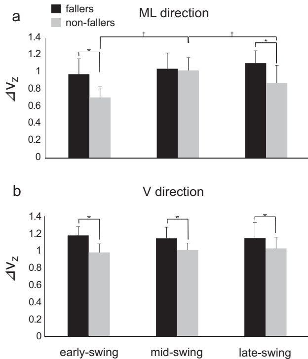
Fig. 4. Averaged synergy index across subjects with standard deviation: Synergy index ( \Delta V_z ) in fallers (black bars) and in non-fallers (grey bars) are shown in ML (a) and V (b) directions. For abbreviation, see the caption for Fig. 2. *Significant differences ( p < 0.05 ) between fallers and non-fallers; †Significant differences ( p < 0.05 ) between phases.
