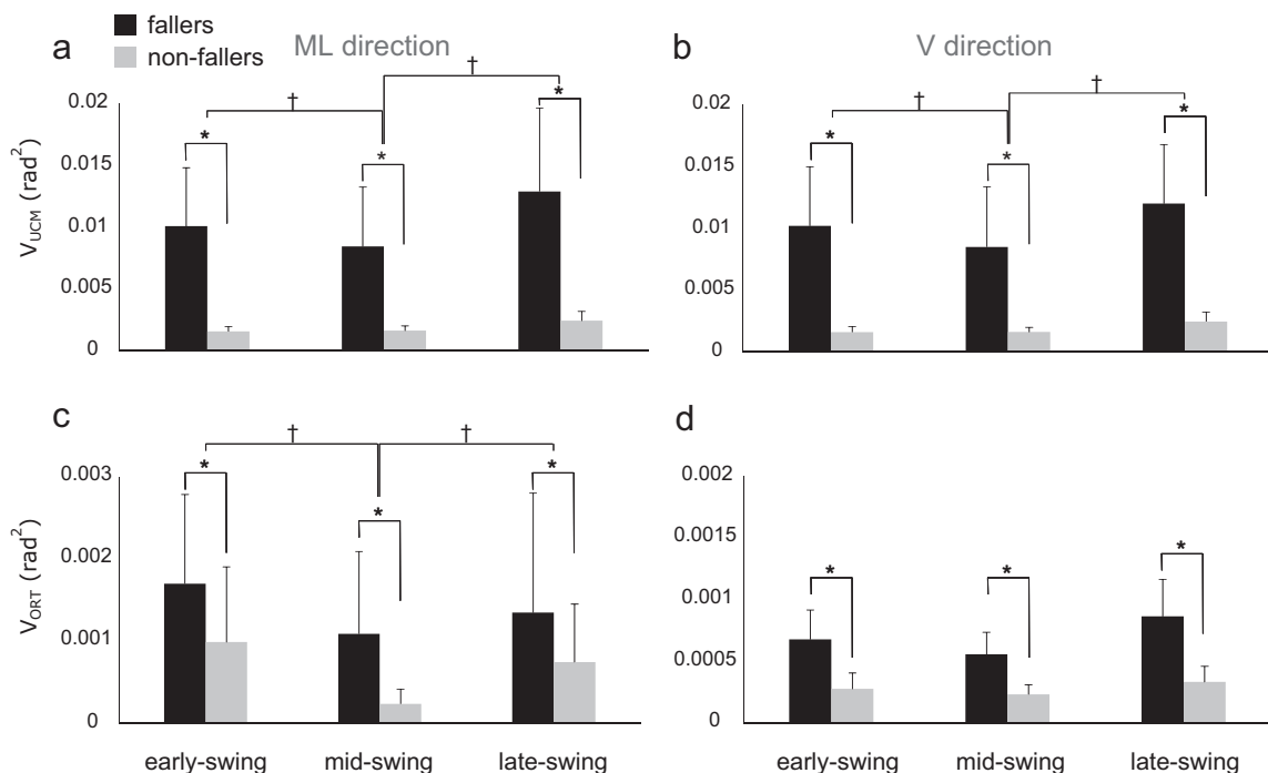
Fig. 3. Averaged variance components across subjects with standard deviation: V_{UCM} (a and b) and V_{ORT} (c and d) in fallers (black bars) and in non-fallers (grey bars) are shown. For abbreviation, see the caption for Fig. 2. *Significant differences ( p < 0.05 ) between fallers and non-fallers; †Significant differences ( p < 0.05 ) between phases.
