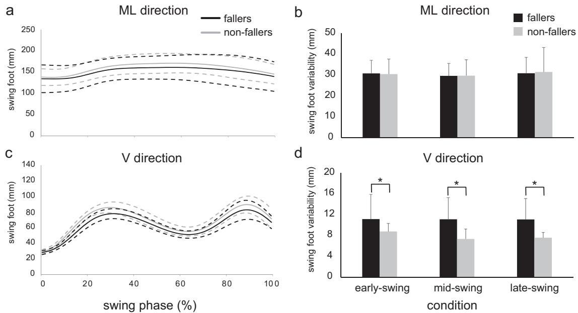
Fig. 2. The averaged time profiles of the swing foot (a and c) and the swing foot variability (b and d) across subjects with standard deviation. Left panels (a and c): the averaged time profiles of the swing foot in the normalized swing phases. The solid lines represent the averaged values, and the dotted lines represent the standard deviations; Right panels (b and d): the swing foot variability for three phases, early-swing, mid-swing, and late-swing. The error bars represent the standard deviations. The indices of the swing foot in fallers (black lines or black bars) and in non-fallers (grey lines and grey bars) are shown in mediolateral (ML) and vertical (V) direction. *Significant differences ( p < 0.05 ) between fallers and non-fallers.
