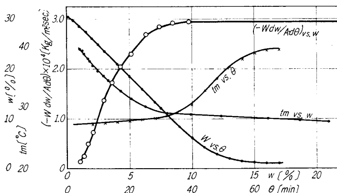
Fig. 1. Drying curve for small sphere. (dia. 0.807 cm, material \text{BaSO}_4 powder (100# pass), t=40^\circ\text{C} , H=0.0148 , u=1.0 m/sec).
