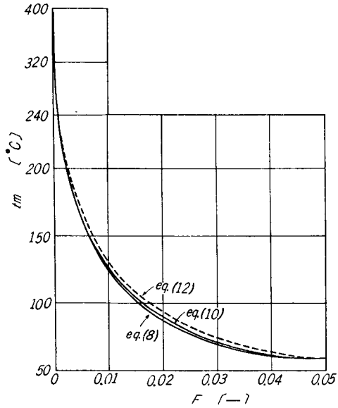
Fig. 8. Relation between water content and material temperature during the falling rate period ( t=400^\circ\text{C} , t_w=60^\circ\text{C} , w_c=0.05 , w_s=0 , c=0.3 ).
