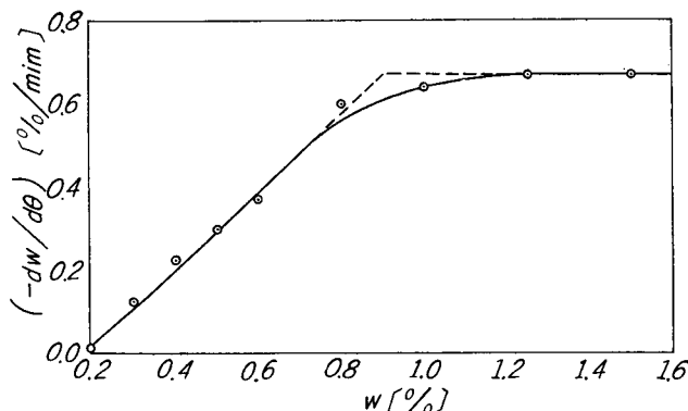
Fig. 2. Drying rate curve for (\text{NH}_4)_2\text{SO}_4 salt in a trough agitator dryer 23 (30 r.p.m, 3 kg-charge, jacket steam press. 1.5 \text{ kg/cm}^2 gauge, wt. basis median dia. 0.3 mm, initial water content w_1=0.06 ).
