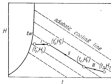
Fig. 15. The approximated change of the air conditions in counter-current flow dryer.
