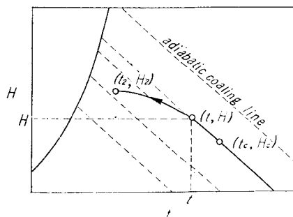
Fig. 11. The change of air conditions in the dryer during the falling rate period. (parallel-current flow)
