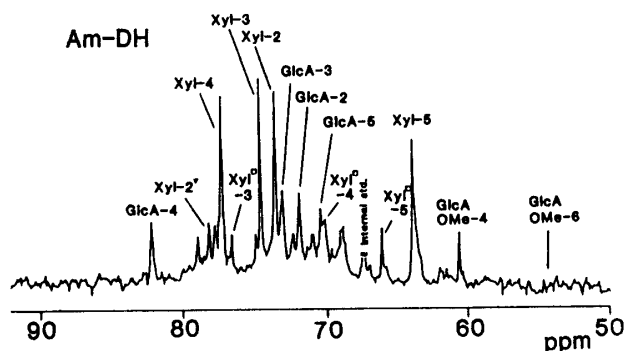
Fig. 35. Carbon-13 n.m.r. spectrum of the acidic fraction (Am-DH) formed from the diazomethane-methylated LCC (C-1-Am) by the action of DDQ.
