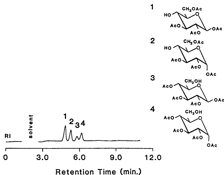
Fig. 23. High performance liquid chromatogram of the partially acetylated D-glucose derivatives on Waters \mu -porasil with n -hexane/ethyl alcohol/acetic acid (200:20:1, v/v/v).
