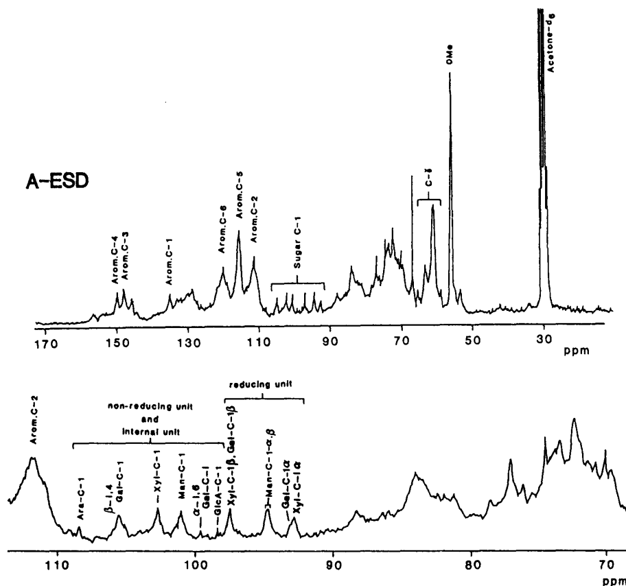
Fig. 14. Carbon-13 n.m.r. spectra of the cellulase-degraded LCC fragments (A-ESD) isolated from the enzymatic digests of the acidic LCC (com-C-1-A) by adsorption chromatography on Toyopearl HW-50F.
