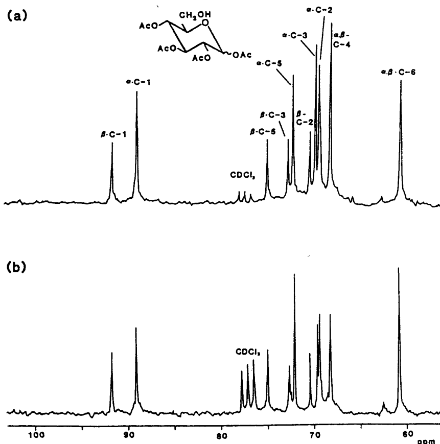
Fig. 25. Carbon-13 n.m.r. spectra of 1,2,3,4-tetra- O -acetyl-D-glucose before and after the DDQ-oxidation in the dichloromethane-water mixture.
