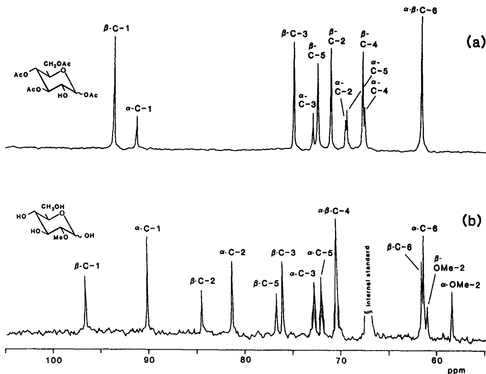
Fig. 30. Carbon-13 n.m.r. spectra of 1,3,4,6-tetra- O -acetyl-D-glucose and its methylated derivative.
