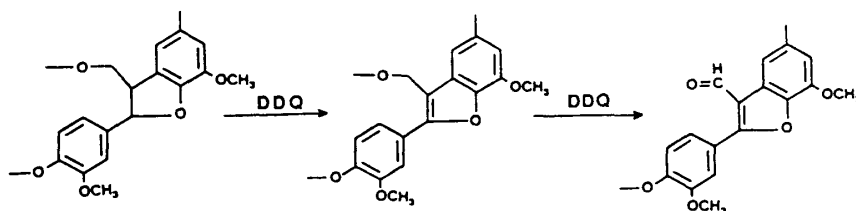
Scheme 3. Oxidation of phenylcoumaran units by DDQ under anhydrous condition.
