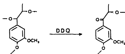
Scheme 1. Oxidation of the benzyl position of phenylpropane units by DDQ.
