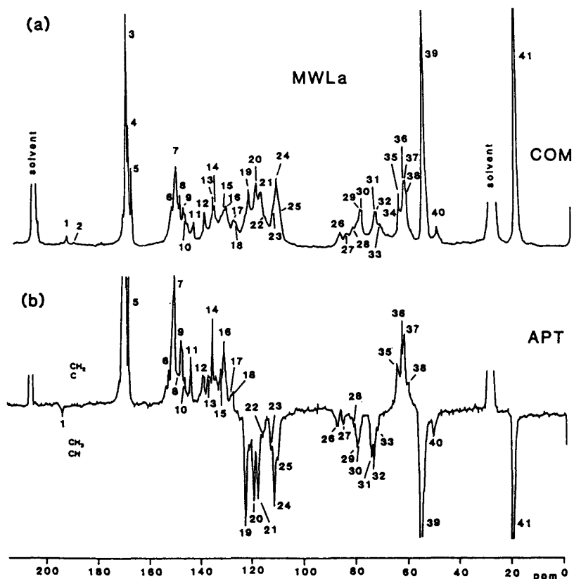
Fig. 17. Carbon-13 n.m.r. spectra of the acetylated milled wood lignin fraction (MWLa) from Pinus densiflora wood.
