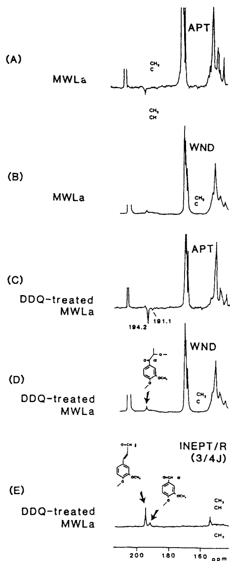
Fig. 19. Carbonyl signals of the acetylated MWL fractions. Notes: (A) Untreated fraction (APT); (B) Untreated fraction (WND); (C) DDQ-treated fraction (APT); (D) DDQ-treated fraction (WND); (E) DDQ-treated fraction (INEPT).
