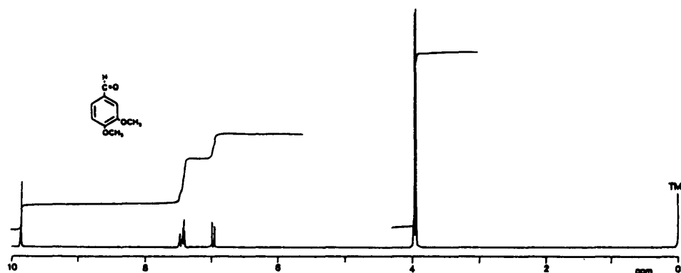
Fig. 33. Proton-n.m.r. spectrum of the aldehyde formed from 3,4-dimethoxybenzyl (1,2,3,4-tetra- O -acetyl)- D -glucuronate by the action of DDQ in the presence of water.
