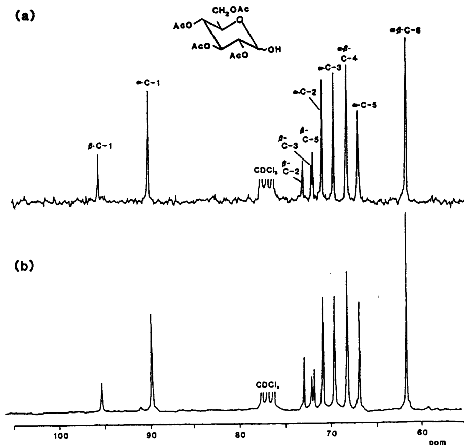
Fig. 27. Carbon-13 n.m.r. spectra of 2,3,4,6-tetra-O-acetyl-D-glucose before and after the DDQ-oxidation in the dichloromethane-water mixture.
