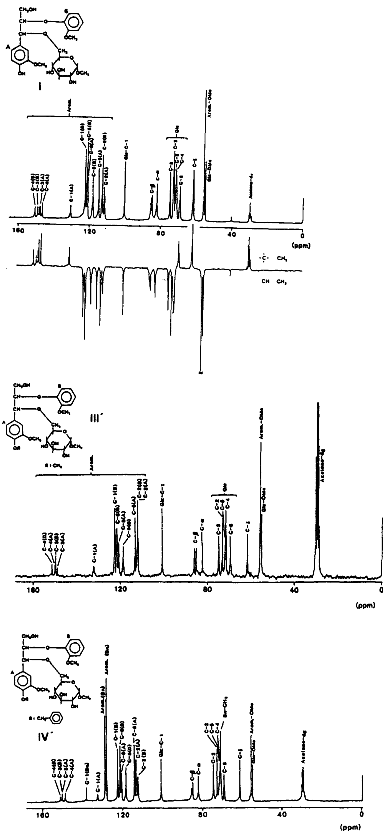
Fig. 15. Carbon-13 n.m.r. spectra of the LCC model compounds.
