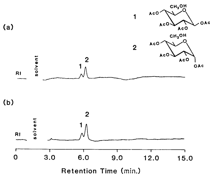
Fig. 24. High performance liquid chromatogram of 1,2,3,4-tetra- O -acetyl-D-glucose before and after the DDQ-oxidation in the dichloromethane-water mixture.
