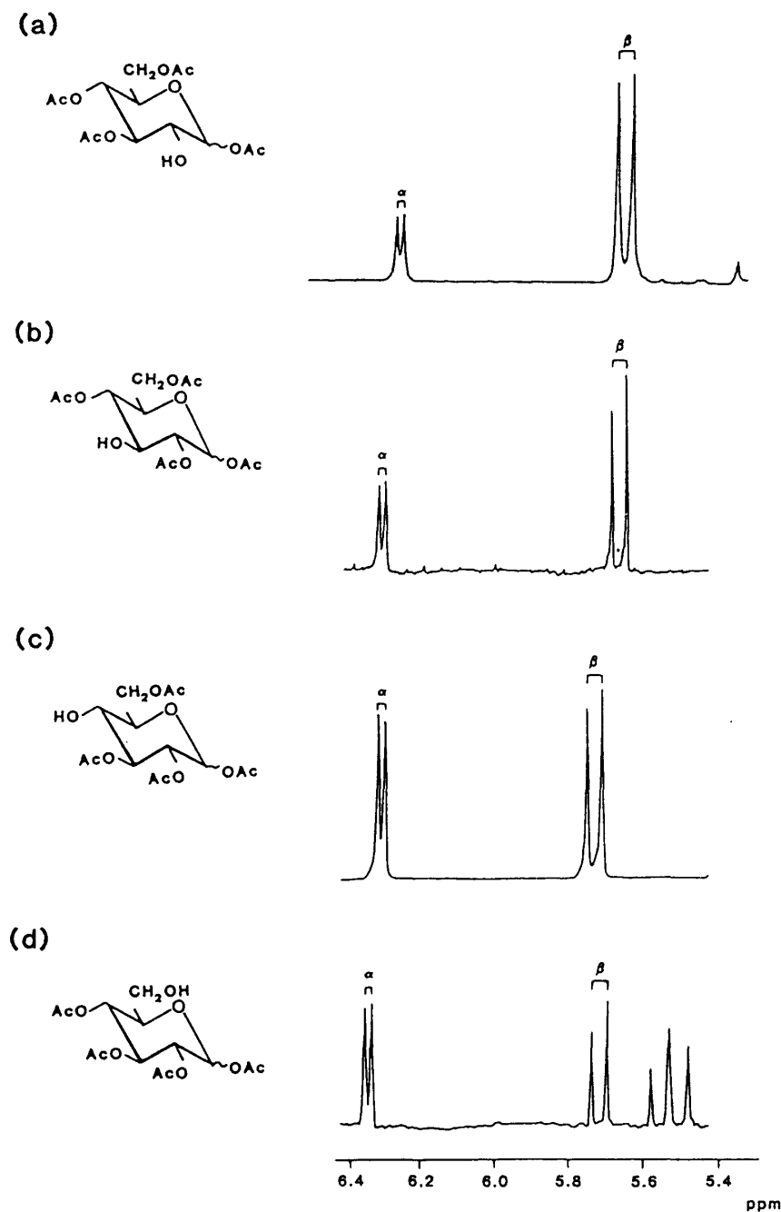
Fig. 22. Proton-n.m.r. spectra of anomeric region of the partially acetylated glucose. Notes: (a) 1,3,4,6-Tetra- O -acetyl-D-glucose; (b) 1,2,4,6-Tetra- O -acetyl-D-glucose; (c) 1,2,3,6-Tetra- O -acetyl-D-glucose; (d) 1,2,3,4-Tetra- O -acetyl-D-glucose.
