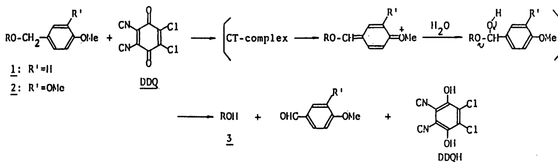
Fig. 16. Oxidative cleavage of benzyl ethers by DDQ in the presence of water.
