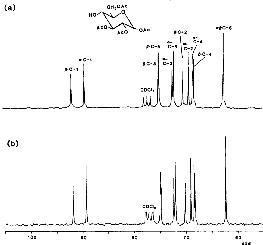
Fig. 26. Carbon-13 n.m.r. spectra of 1,2,3,6-tetra-O-acetyl-D-glucose before and after the DDQ-oxidation in the dichloromethane-water mixture.
