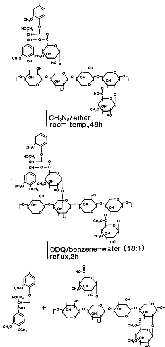
Fig. 34. Schematic representation of the new method to prove the existence of ester linkages between lignin and 4- O -methylglucuronic acid residue in hemicelluloses.
