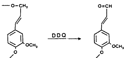
Scheme 2. Oxidation of the \gamma -position of conjugated arylpropene units by DDQ.
