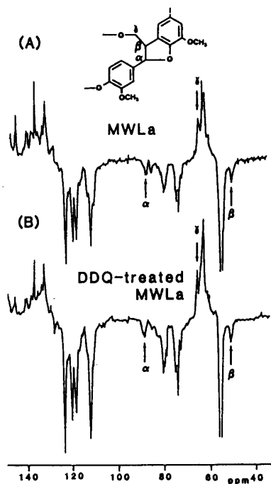
Fig. 20. Signals of carbon atoms in the phenylcoumaran units before and after the DDQ-oxidation. Notes: (A) Untreated fraction; (B) DDQ-treated fraction.
