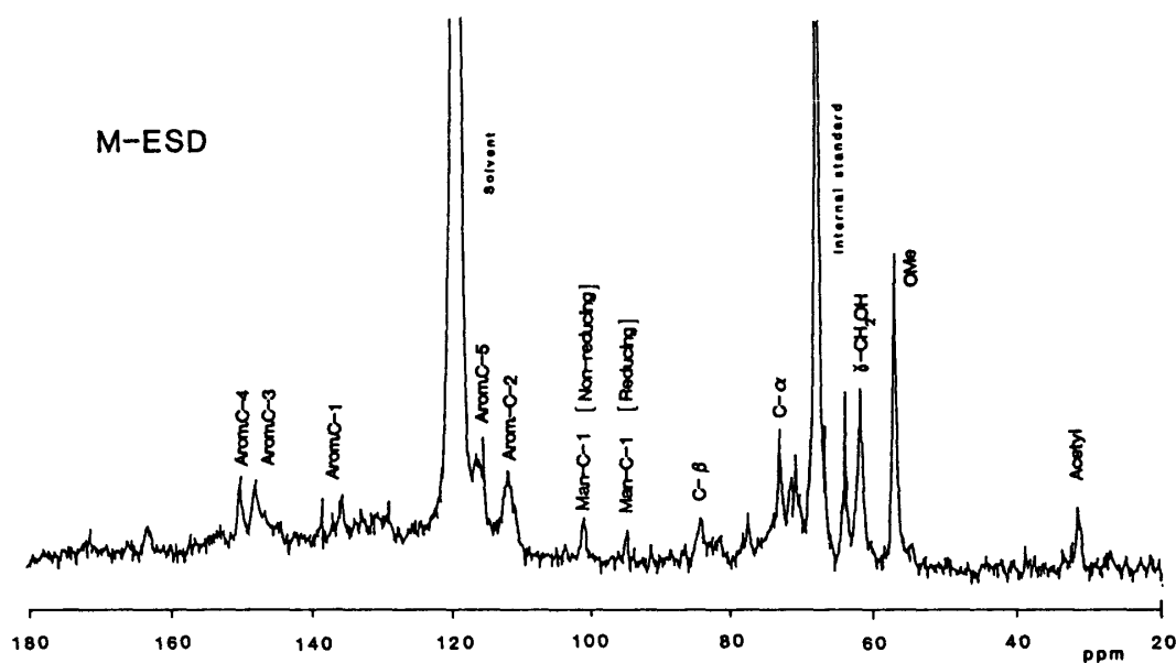
Fig. 13. Carbon-13 n.m.r. spectrum of the cellulase-degraded LCC fragments (M-ESD) isolated from the enzymatic digests of the lignin-acetylglucomannan complex (nor-C-1-M) by adsorption chromatography on Toyopearl HW-40S.
