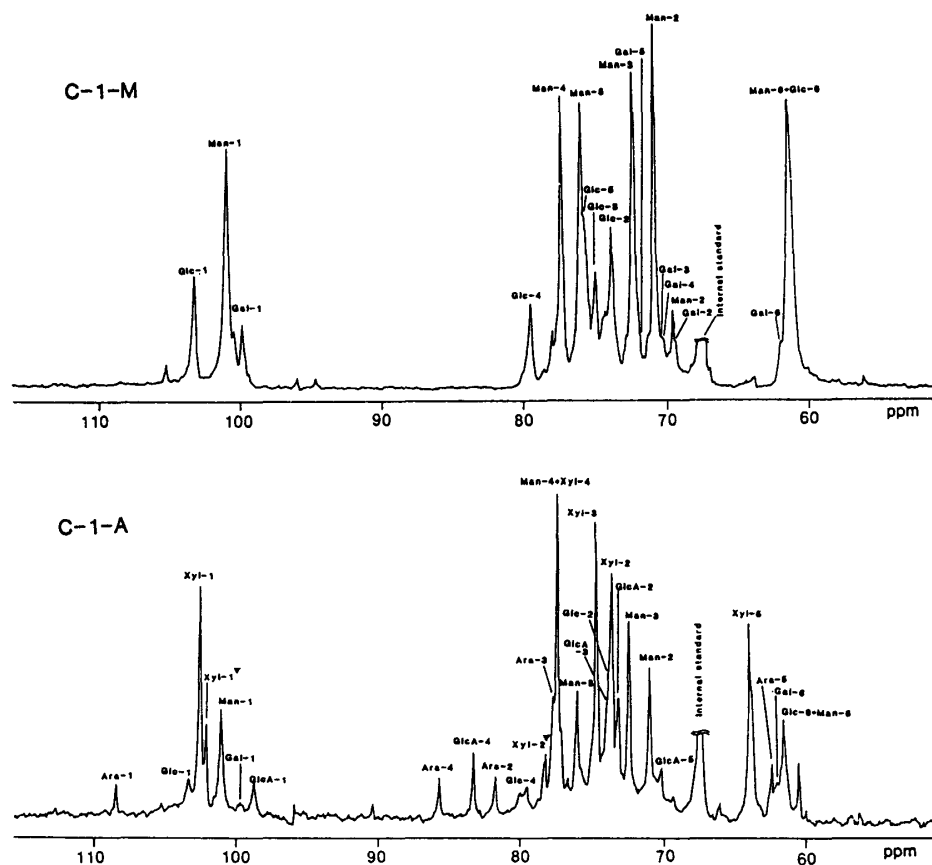
Fig. 2. Carbon-13 n.m.r. spectra of the LCC-WE fractions. Notes: Chemical shifts in ppm are expressed down-field from TMS with dioxane as an internal standard (67.4 ppm from TMS). ▲--- This signal was due to the C-2 substituted xylopyranosyl residues.
