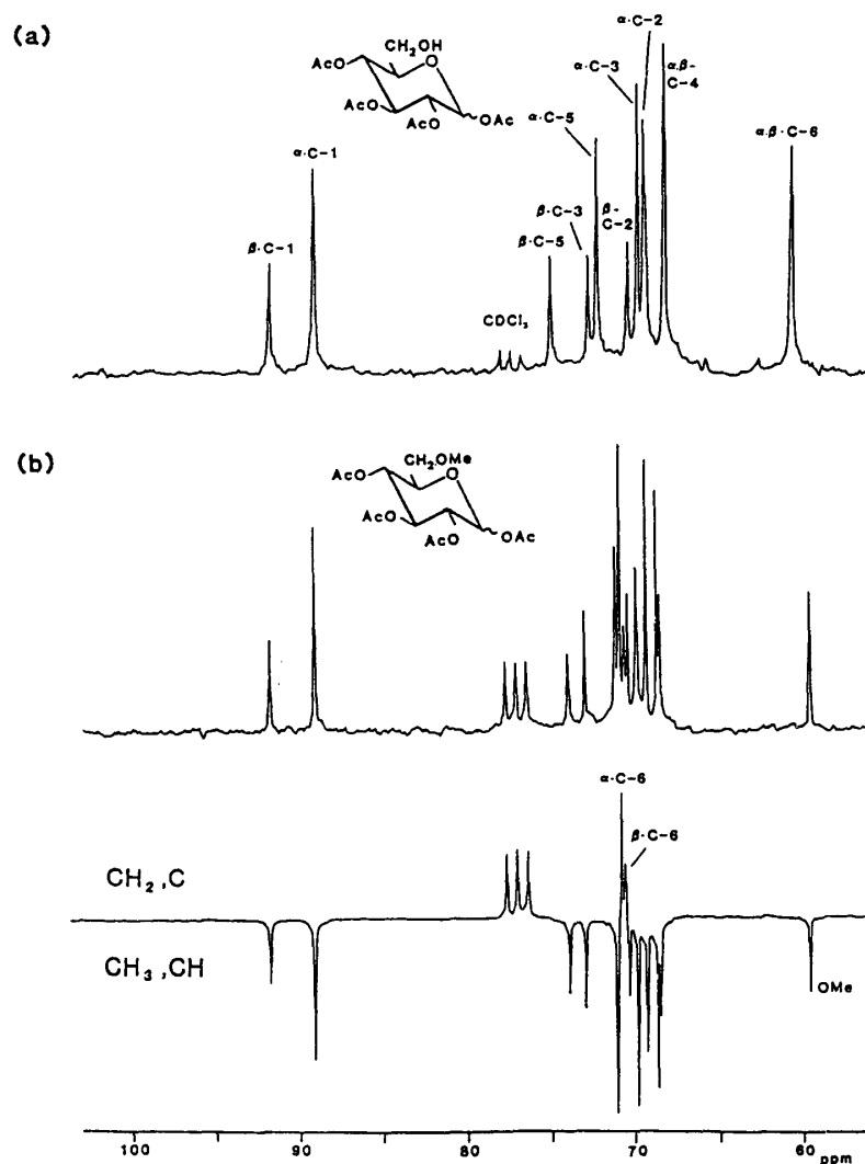
Fig. 29. Carbon-13 n.m.r. spectra of 1,2,3,4-tetra- O -acetyl-D-glucose and its methylation products by the method of Prehm. Notes: (a): 1,2,3,4-tetra- O -acetyl-D-glucose; (b): Methylation products from 1,2,3,4-tetra- O -acetyl-D-glucose by the method of Prehm.
