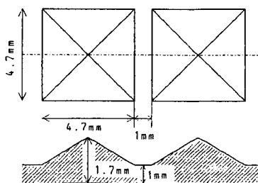
Fig.3 Roughness Element
