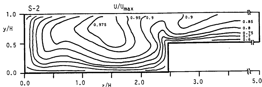
Fig.8 Isovels of Primary Mean Velocity U
