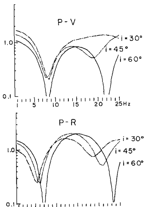
Fig. 5. Vertical and radial components of transfer functions for P waves. Half-space parameters are; V_p = 4.66 km/sec, V_s = 2.45 km/sec, \rho = 2.5 gr/cm 3 and the depth of observational point = 140 m.
