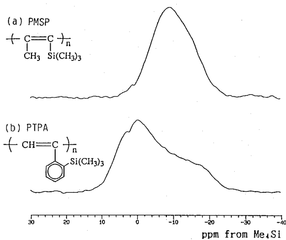
Fig. 8. CP/DD 29 Si NMR spectra obtained for PMSP and PTPA without MAS at room temperature.
