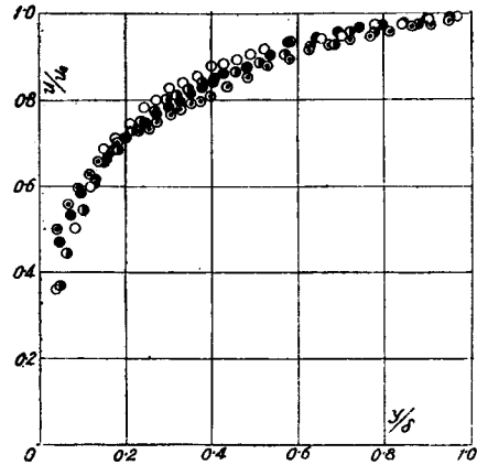
Fig. 10. Velocity Distribution. Rough plate with grooves. p = 8 mm.
