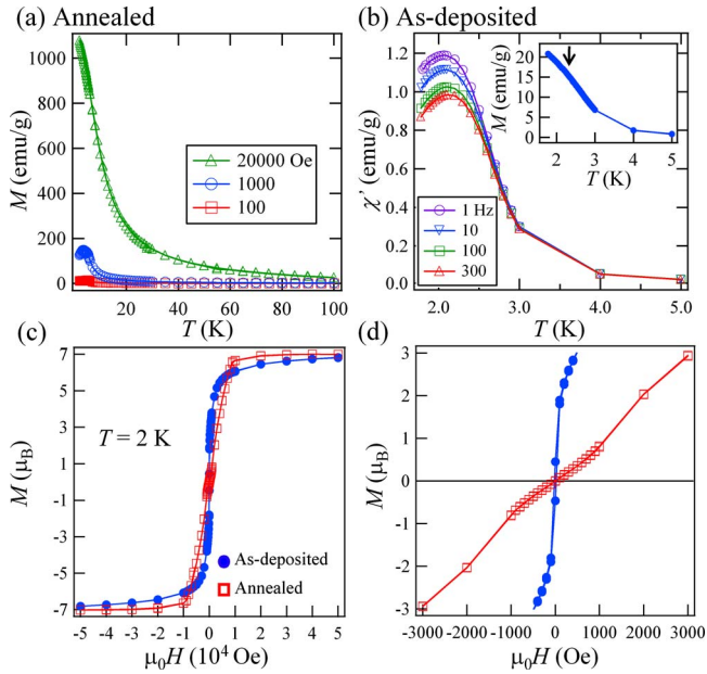
FIG. 4. (Color online) (a) M - T curves for annealed \text{EuTiO}_3 thin film at H_{dc}=100 (open squares), 1000 (open circles), and 20 000 Oe (open triangles) applied along the \langle 100 \rangle direction. (b) \chi' - T curves for the as-deposited \text{EuTiO}_3 thin film at H_{ac}=3 Oe and H_{dc}=0 Oe. The ac frequencies are 1, 10, 100, and 300 Hz. The inset represents the low-temperature data of the M - T curve for as-deposited film as shown in Fig. 3(b). The arrow denotes an inflection point. (c) Magnetic field ( \mu_0 H ) dependence of M at 2 K for the as-deposited (closed circles) and annealed (open squares) \text{EuTiO}_3 thin films. (d) Enlarged view of (c).
