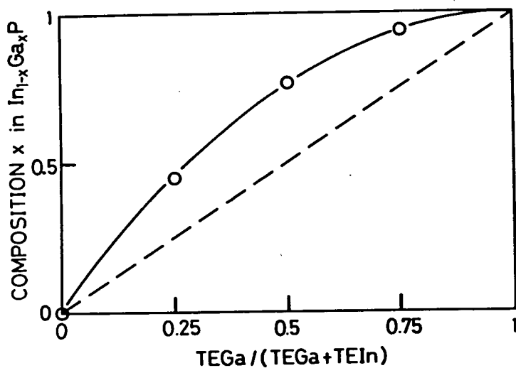
Fig. 2.6. Dependence of composition x in \text{In}_{1-x}\text{Ga}_x\text{P} on flux ratio of TEGa/(TEGa+TEIn). (640°C, TEIn=0.029, \text{PH}_3 =1.00 sccm).
