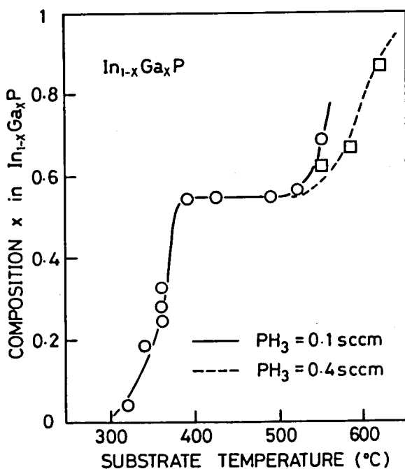
Fig. 3.11. Temperature dependence of epilayer composition x in \text{In}_{1-x}\text{Ga}_x\text{P} . (TEIn=0.016, TEGa=0.020 sccm).
