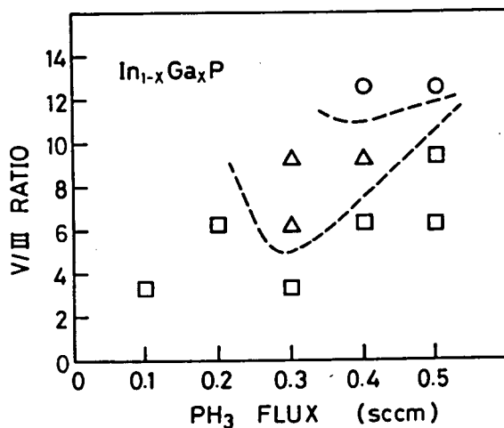
Fig. 3.35. V/III ratio and phosphine flux dependence of surface morphology grown at 585^{\circ}\text{C} . Smooth surface ( \circ ), complex defect ( \triangle ), and indium droplet ( \square ). Broken lines represent boundary of surface morphology.
