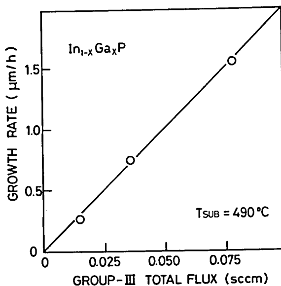
Fig. 3.14. Dependence of growth rate on group-III total flux of \text{TEGa} + \text{TEIn} .
