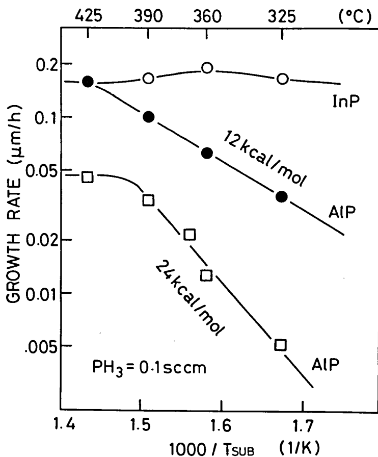
Fig. 4.7. Arrhenius plot of growth rates of quasi-binaries (InP (○) and AlP (●)) in InAlP epitaxy (TEIn=0.0073, TEAl=0.016 sccm), and of AlP (□) in binary growth (TEAl=0.016 sccm), at lower temperatures.
