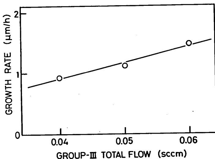
Fig. 2.5. Dependence of growth rate on group-III total flow of TEGa+TEIn. (640°C, TEIn/TEGa=0.30, \text{PH}_3 =1.00 sccm).
