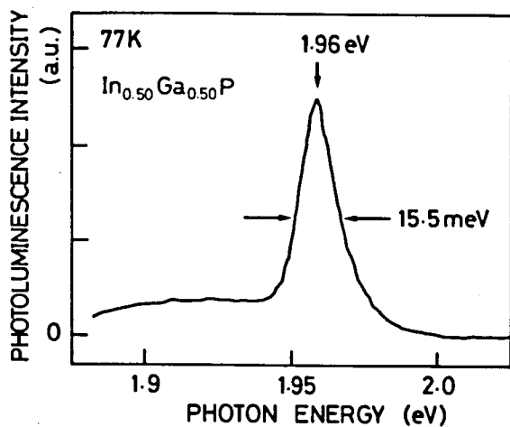
Fig. 3.21. Band-edge PL peak of typical \text{In}_{0.5}\text{Ga}_{0.5}\text{P} epilayer grown at 490°C.
