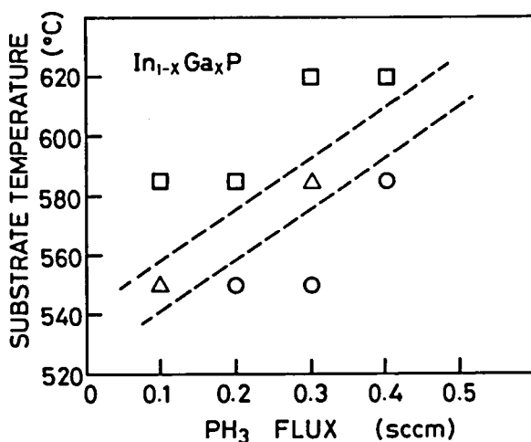
Fig. 3.34. Temperature and phosphine flux dependence of surface morphology grown with \text{TEGa}=\text{TEIn}=0.016 sccm. Smooth surface ( \circ ), complex defect ( \triangle ), and indium droplet ( \square ). Broken lines represent boundary of surface morphology.
