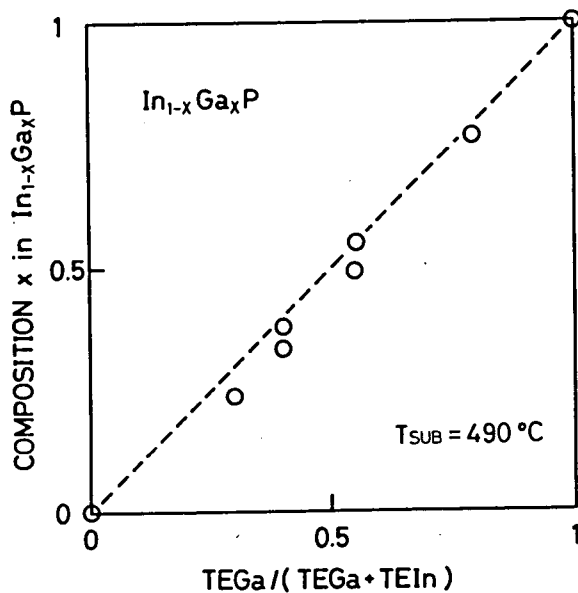
Fig. 3.15. Dependence of epilayer composition x in \text{In}_{1-x}\text{Ga}_x\text{P} on flux ratio of \text{TEGa}/(\text{TEGa} + \text{TEIn}) .
