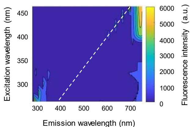
Fig. S5 An example of excitation–emission matrix of sweet pepper fruit pericarps. The white-dashed line, a linear-like wavelength function, indicates the Raman band (not fluorescence). At 360 nm excitation, the Raman band was observed near 550 nm and was excluded from the analysis (described in the experimental section). Strong red emission (a typical emission band of chlorophyll) was observed in the 400–460 nm excitation range.
