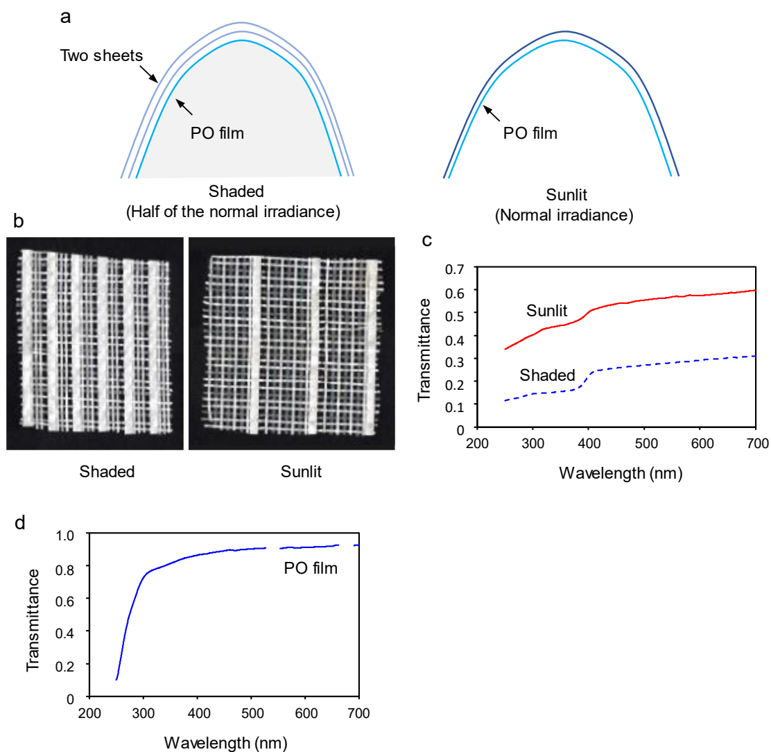
Fig. S1 (a) Schematic of a cultivation house with different solar exposures. (b) Photographs of the shading material. (c) Transmission spectra for each calculated cultivation condition (irradiance with polyolefin (PO) film is regarded as 1.0). (d) Transmission spectra of the polyolefin film. Spectral distortions were removed at 550 and 670 nm due to the device's stability.
