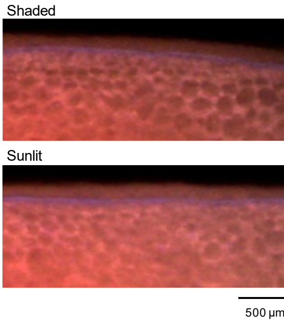
Fig. 2 Fluorescence microscopy images of the pericarp cross-section samples of sweet pepper at 365 nm excitation. Two groups are shown: high (normal) and low (half of the normal) sunlight exposure. The black-red interface in the upper region is the surface of the fruit.
