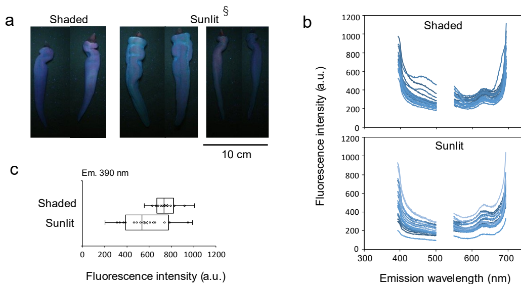
Fig. 1 (a) Fluorescence image of sweet pepper at 365 nm excitation. Two types of fluorescence patterns were observed under sunlit conditions. (b) Fluorescence spectrum at 360 nm excitation. (c) 390 nm fluorescence emission intensity (360 nm excitation). Two groups are shown: high (normal) and low (half of the normal) sunlight exposure. n = 20 for each group. Fluorescence intensities at \sim 550 nm and > 695 nm were excluded (see the experimental section). (a) § Two patterns were observed for the sunlit conditions: bright- and dark-fluorescent sweet peppers. (b) No excitation light was observed above 390 nm. (c) The average values for the two conditions were significantly different ( P < 0.05 ).
