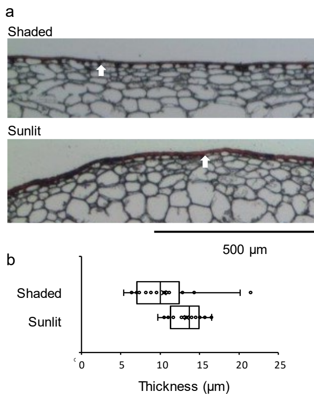
Fig. 3 (a) Microscopic images of Oil Red O-stained cuticle. The cuticle is stained red (white arrows). (b) Thickness of the epidermal cell wall. Two groups are shown: high (normal) and low (half of the normal) sunlight exposure. n = 20 for each group. (b) The average values for the two conditions were significantly different ( P < 0.05 ).
