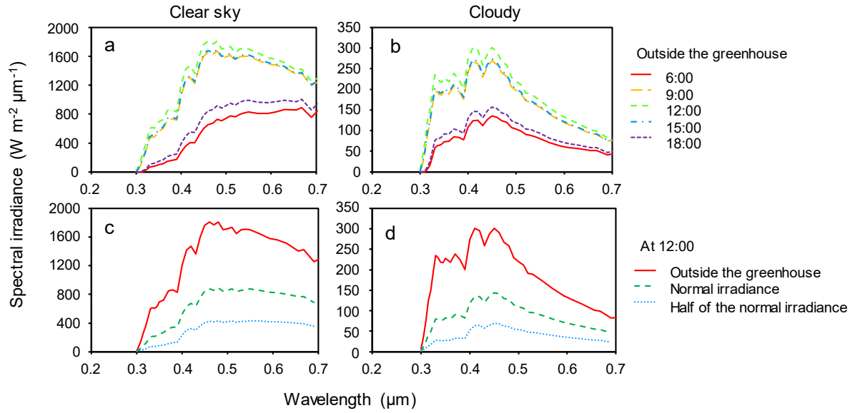
Fig. A1 Spectral irradiance as a function of time and geographic coordinates. The spectral irradiance, as of 15 July 2021, at Kameoka, Kyoto, Japan (N 35.01°, E 135.56°), was calculated by the Bird model [5] and the measured transmission of the polyolefin film and shading materials. The calculation programme is available online under the permission of the National Renewable Energy Laboratory, United States Department of Energy [6]. (a, b) Spectral irradiance at 9, 12, 15 and 18:00. (a) Clear sky and (b) cloudy days. (c, d) Spectral irradiance at noon for outside, sunlit and shaded greenhouse conditions. (c) Clear sky and (d) cloudy days.
