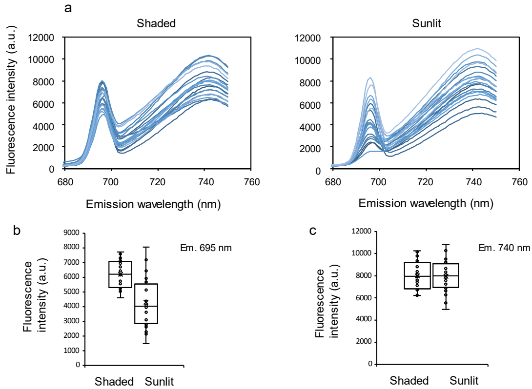
Fig. S2 (a) Red and near-infrared fluorescence spectra of sweet peppers at 460 nm excitation. (b) Red fluorescence intensity (695 nm emission) and (c) near-infrared fluorescence intensity (740 nm emission). Two groups are shown: high (normal) and low (half of the normal) solar exposure. Twenty samples were selected for each group. (b) The average values for the two conditions were significantly different ( P < 0.05 ).
