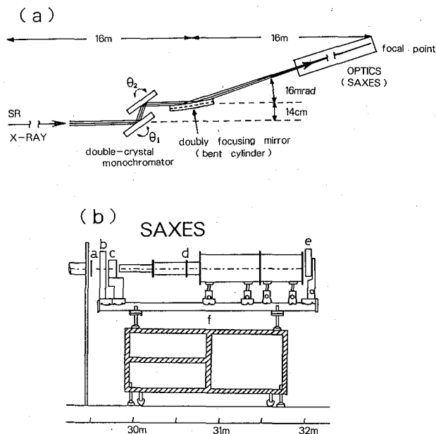
Fig. 1 (a) Optics of BL-10C consisting of a double crystal monochromator and a bentcylindrical mirror. (b) Schematic drawing of the small-angle X-ray scattering equipment for solutions(SAXES). a; the exit window of X-ray beam, b; the third slit assembly, c; specimen holder, d; vacuum pipe, e; detector(PSPC), and f; double optical rails.
