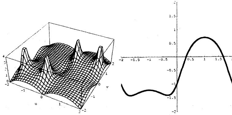
Figure 3: Left: Absolute value of x^{(+)}(uK + i v K') in its fundamental domain -2 \leq u \leq 2 and -2 \leq v \leq 2 . There are two poles on the line \Im t = K' and other two poles on the line \Im t = -K' . Right: Value of 1/x^{(+)}(uK + i K') for -2 \leq u \leq 2 . Two zeros correspond to the two poles on the line \Im t = K' in the left picture.
