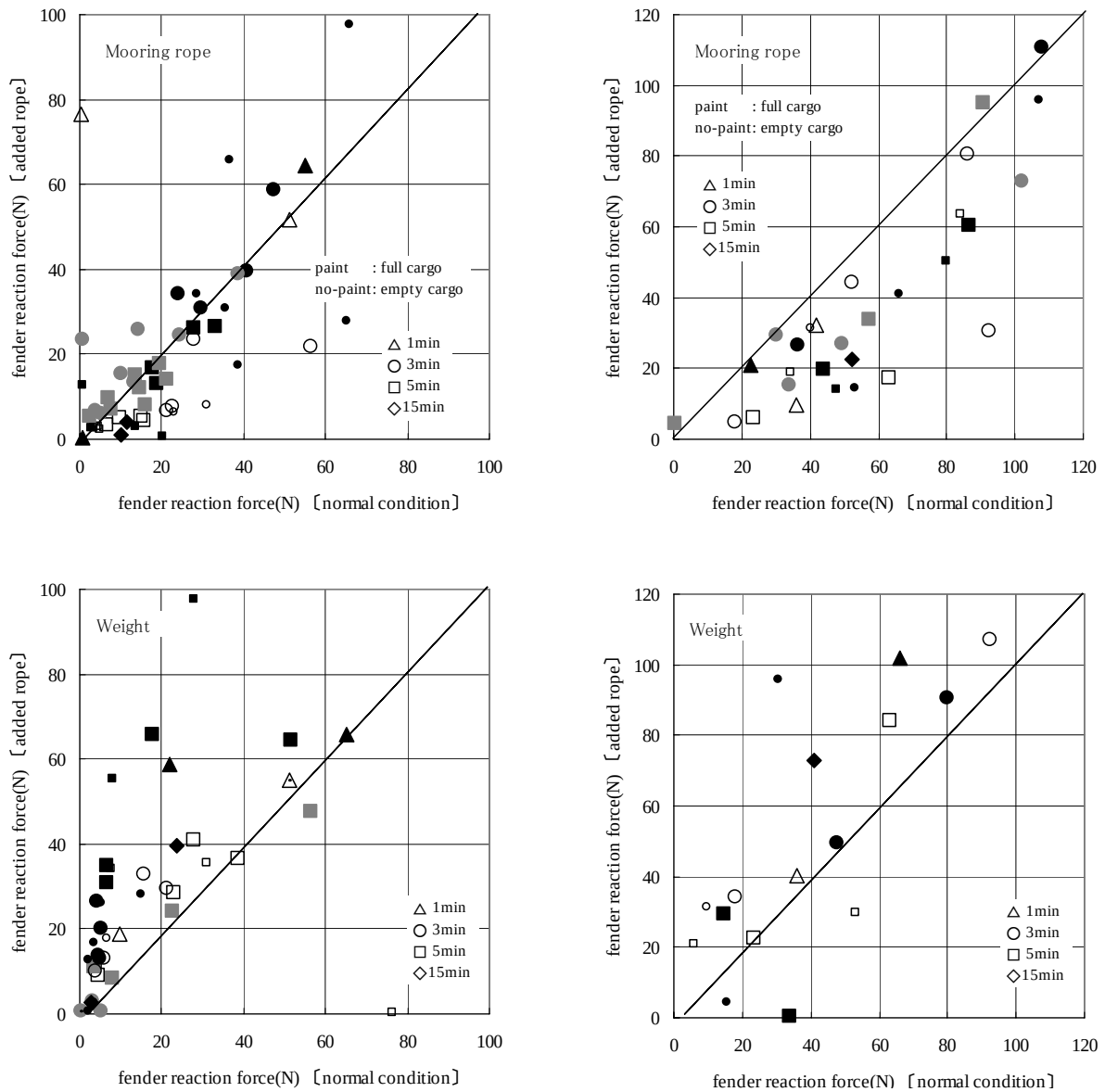
Fig.9 The relationship of fender reaction load that compare with some condition
