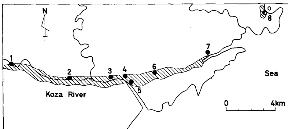
Fig. 1. Showing the localities of the dikes which are composed of liparite and granite porphyry. 1; Kurozu, 2; Oyanagi, 3; Tsukinose, 4; Utsugi, 5; Takaike, 6; Sabe, 7; Uragami, 8; Taiji.
