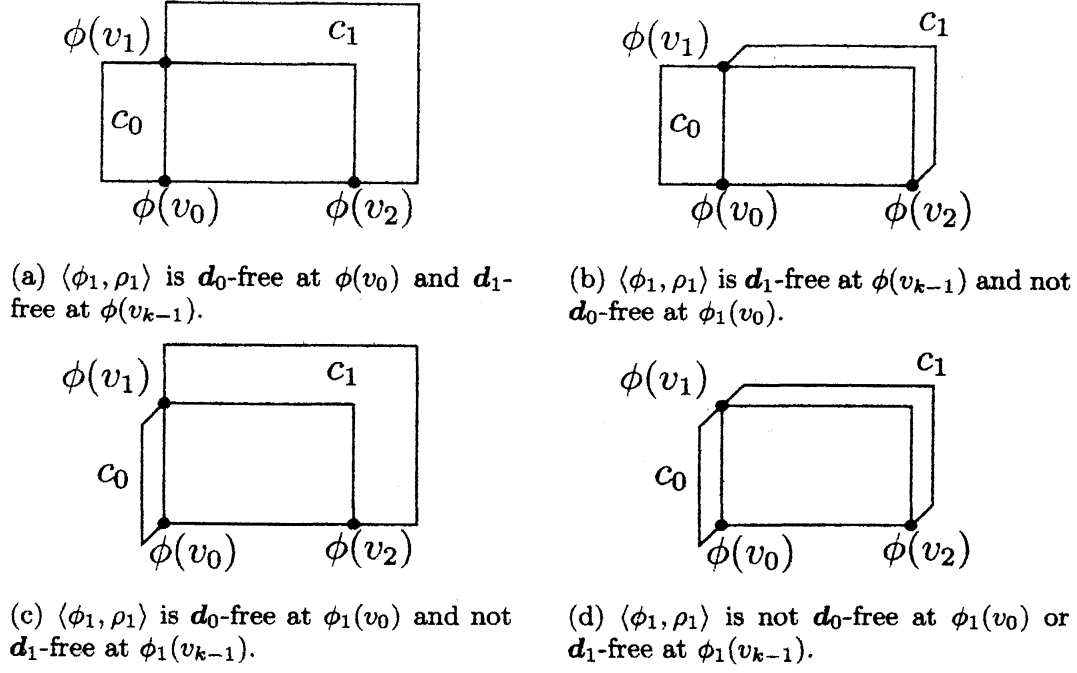
Figure 7: Drawing of child faces of f in Case 1-1.
