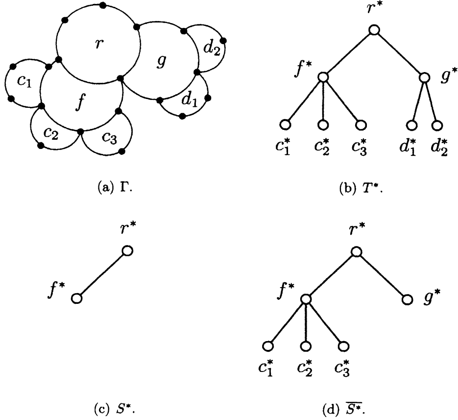
Figure 1: Example of an outerplane graph \Gamma , rooted tree T^* , subtrees S^* and \overline{S^*} of T^* .
