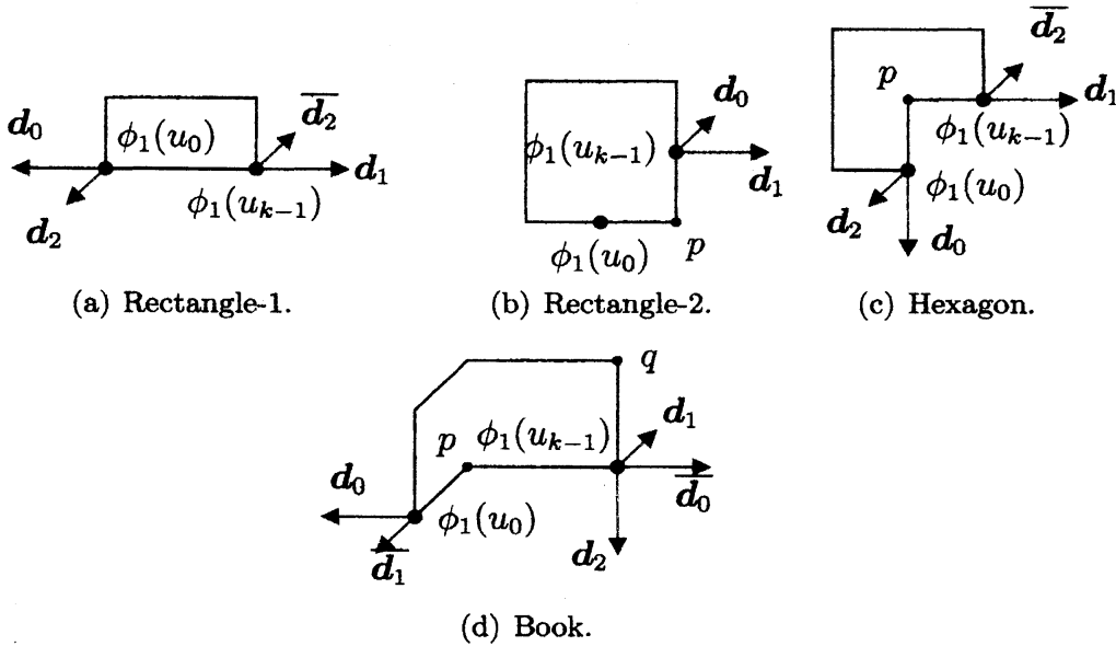
Figure 5: Directions for drawing of face f .
