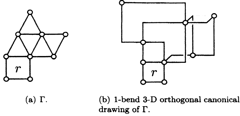
Figure 4: Example of \Gamma and 1-bend 3-D orthogonal canonical drawing of \Gamma .
