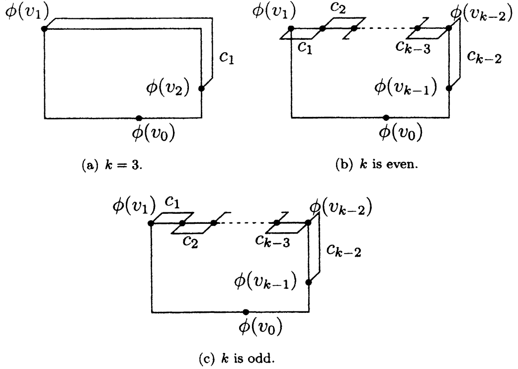
Figure 10: Drawing of child faces of f in Case 2.
