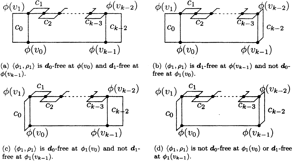
Figure 9: Drawing of child faces of f in Case 1-3.
