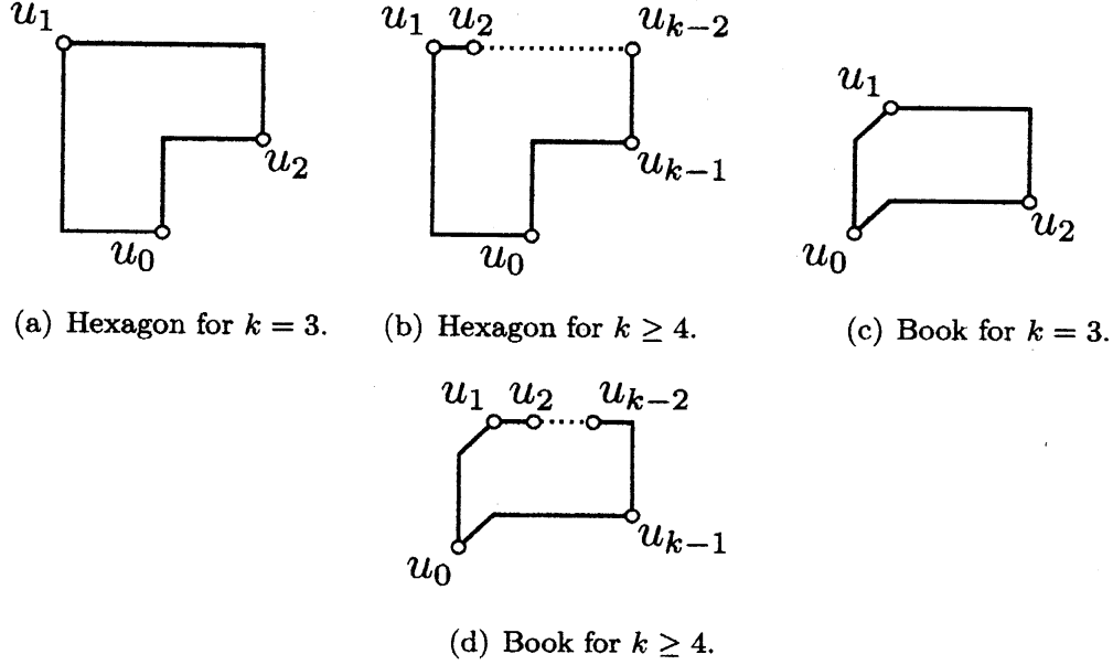
Figure 3: Hexagon and Book.
