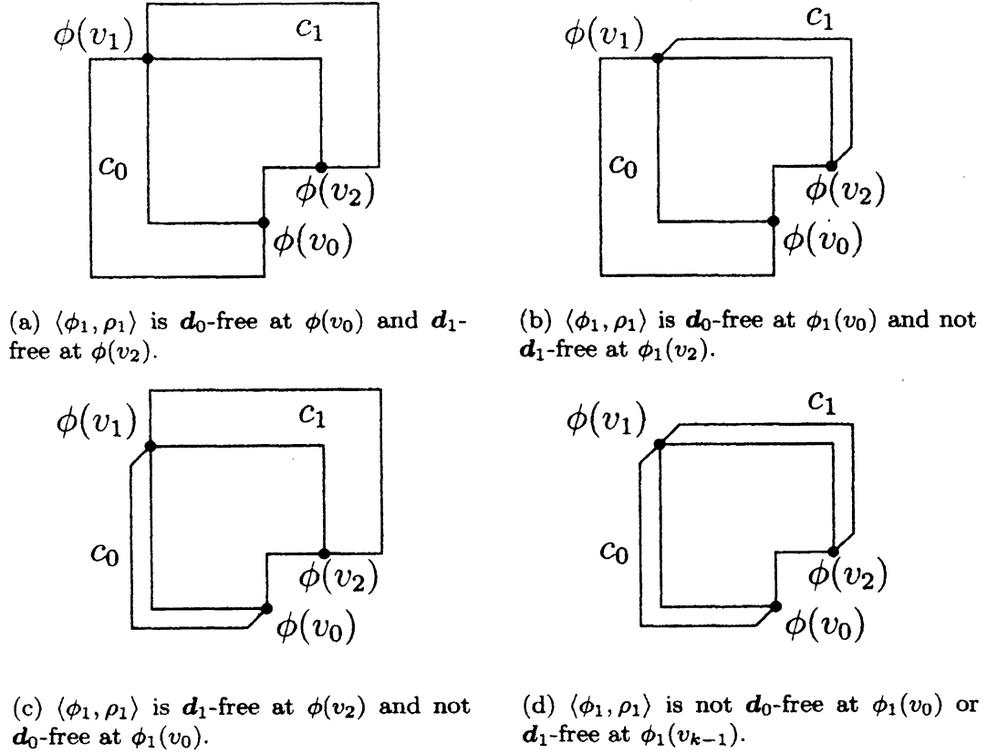
Figure 11: Drawing of child faces of f in Case 3-1.
