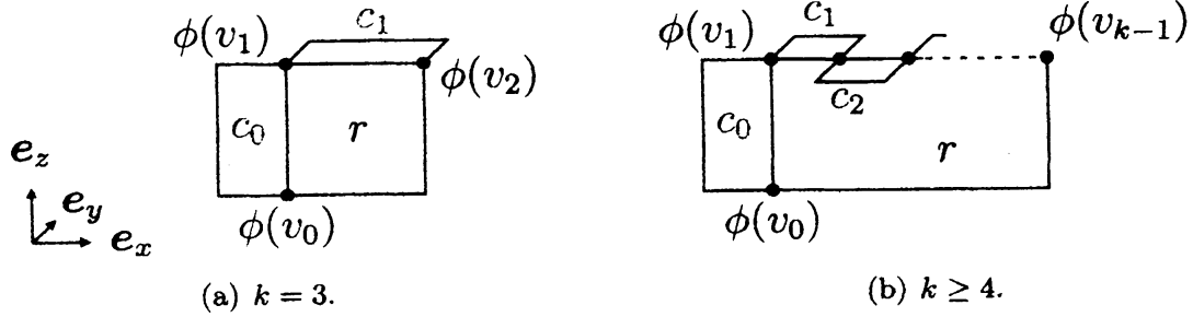
Figure 6: Drawing of initial case.
