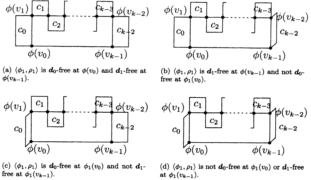
Figure 8: Drawing of child faces of f in Case 1-2.
