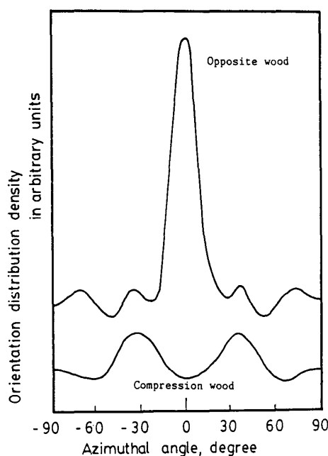
Fig. 20. Orientation distribution of cellulose crystallites in Pinus densiflora .
