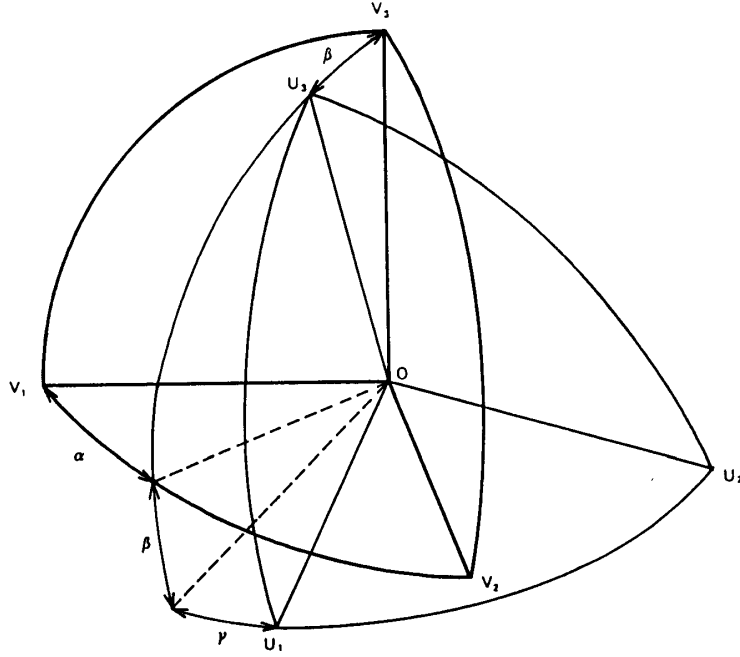
Fig. 24. Relationship between two Cartesian coordinate systems, \mathbf{O-U_1U_2U_3} and \mathbf{O-V_1V_2V_3} . \alpha , \beta , and \gamma are Euler angles.
