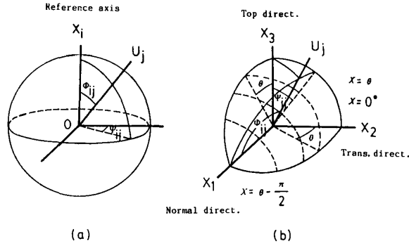
Fig. 14. Spherical coordinates specifying polar angle \Phi_{ij} and azimuthal angle \Psi_{ij} of a reciprocal lattice vector with respect to a reference axis X_i .
