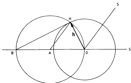
Fig. 5. Schematic representation of Laue condition.
