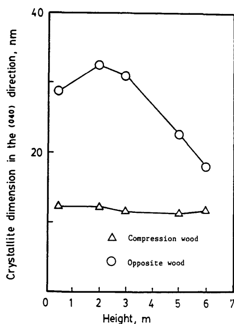
Fig. 22. Crystallite dimension parallel to (040) plane of cellulose crystallites in Pinus densiflora .
