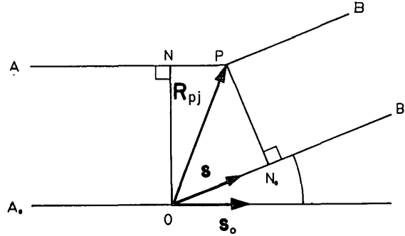
Fig. 3. Path differences between x-rays diffracted at points \mathbf{O} and \mathbf{P} .
