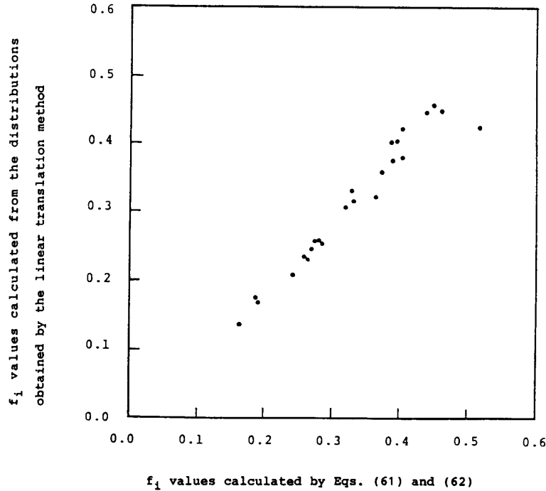
Fig. 29. Relationship between observed and theoretical f_i values.
