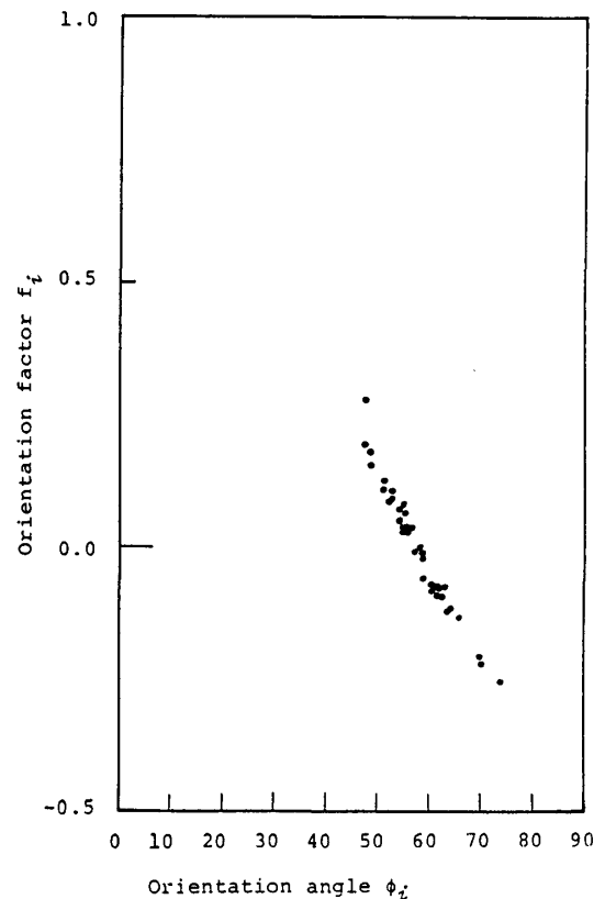
Fig. 32. Relationship between orientation factors and averaged orientation angles.
