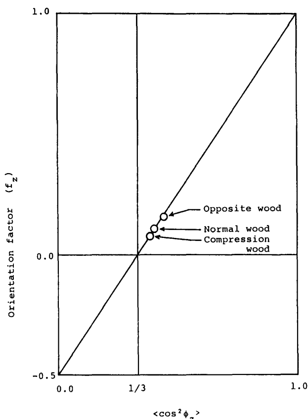
Fig. 31. Relationship between orientation factors and orientation functions.
