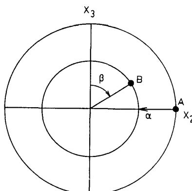
Fig. 10. Schematic representation of location of a pole ( \alpha=0^\circ , \beta=90^\circ ).
