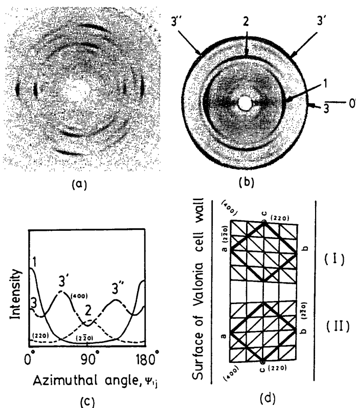
Fig. 15. X-ray diagrams of wall of Valonia macrophysa Kützing and the disposition of basal planes: (a) beam normal to wall surface (through-view pattern); (b) beam parallel to wall surface (edge-view pattern); (c) relative values of I(\Phi, \Psi) with respect to azimuthal angle \Psi_{ij} for edge-view pattern starting from the equator, marked 0 in (b). (d) Disposition of the basal planes of the two unit cells necessary to explain (b) and (c).
