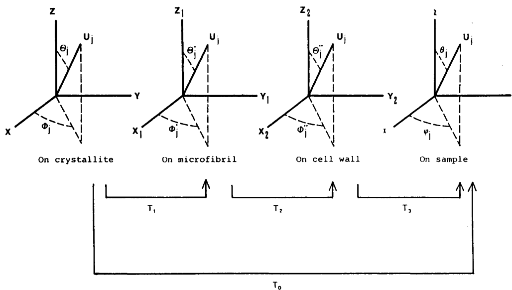
Fig. 23. Cartesian coordinate systems fixed on orientational units in wood and the linear translations between them.
