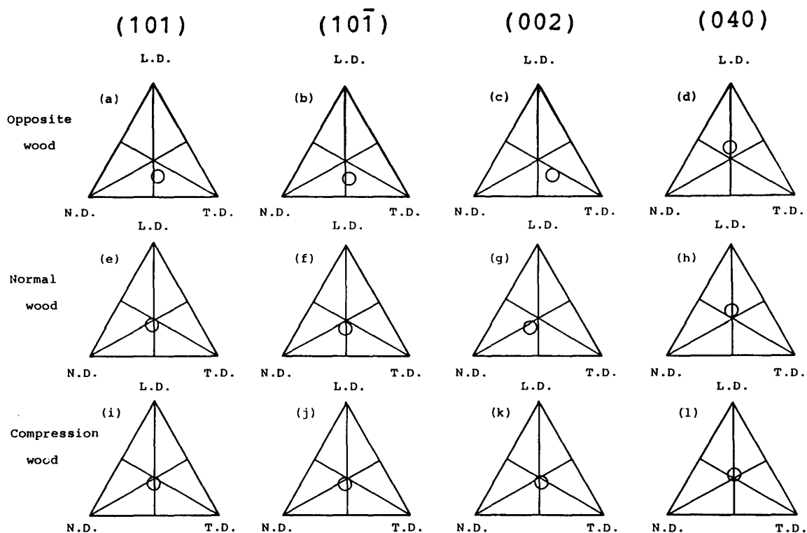
Fig. 30. Equilateral triangular coordinate plots of average directional squared cosines for distributions of cellulose crystallites in Pinus densiflora wood.
