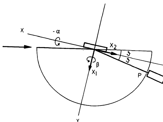
Fig. 11. Geometry of reflection technique for pole figure measurements.
