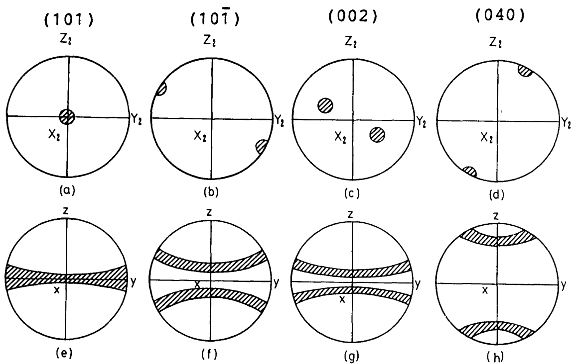
Fig. 26. Ideal pole density distributions of cellulose crystallites in wood and cell walls in the case of planar orientation.
