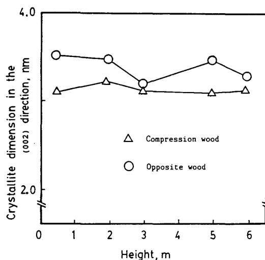
Fig. 21. Crystallite dimension parallel to (002) plane of cellulose crystallites in Pinus densiflora .
