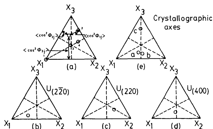
Fig. 17. Equilateral triangle diagrams representing degree of biaxial orientation of the longitudinally aligned Valonia cellulose crystallites in terms of three quantities, \langle \cos^2 \phi_{1j} \rangle , \langle \cos^2 \phi_{2j} \rangle , and \langle \cos^2 \phi_{3j} \rangle .
