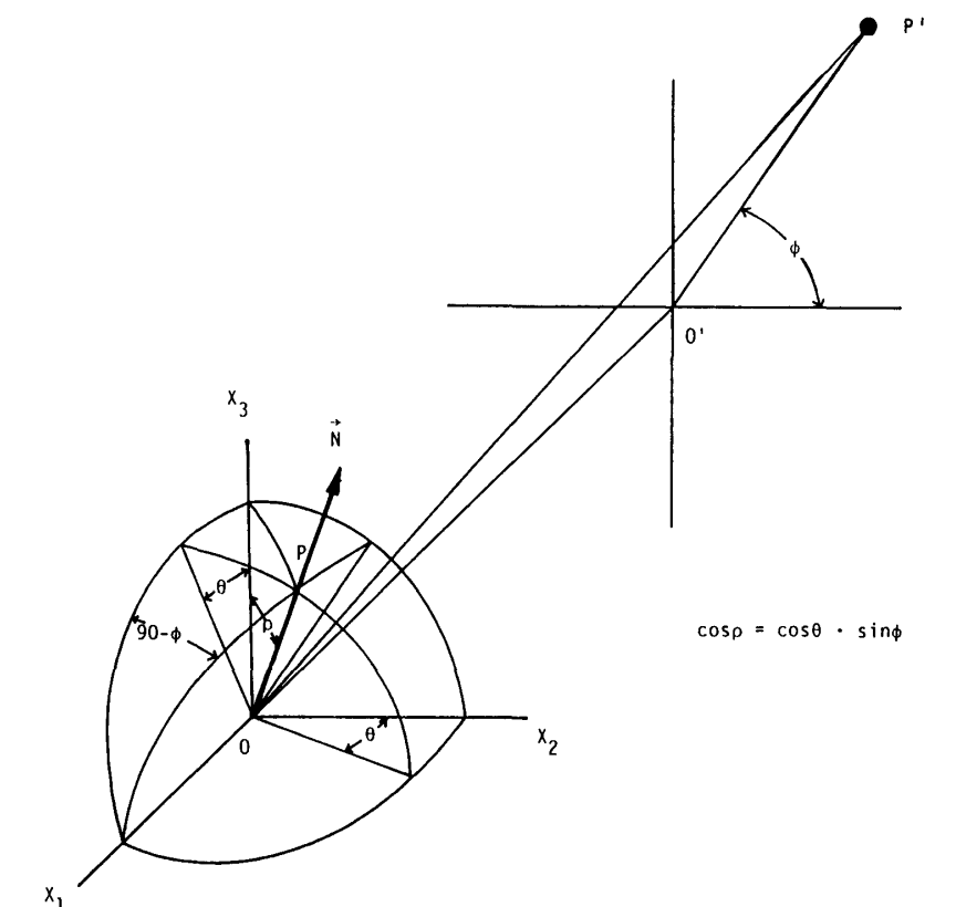
Fig. 6. Schematic representation of relationship between plane-normal and x-ray fiber diagram.
