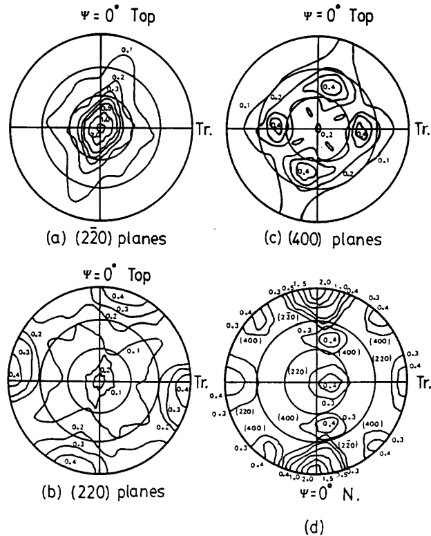
Fig. 16. Projection of hemisphere on X_2X_3 plane showing pole distribution for: (a) (2\bar{2}0) planes; (b) (220) planes; (c) (400) planes; and (d) projection of hemisphere on X_1X_2 plane showing pole distribution for all planes.
