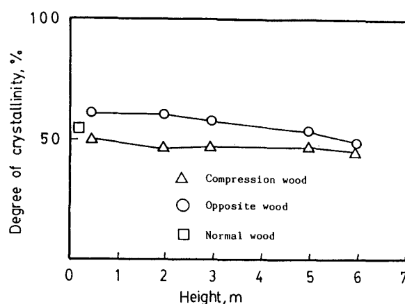
Fig. 19. Degree of crystallinity for cellulose crystallites in Pinus densiflora .
