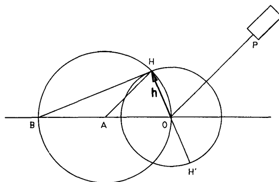
Fig. 7. Geometrical representation of certain reciprocal vector for which x-ray diffraction can be observed at point \mathbf{P} .
