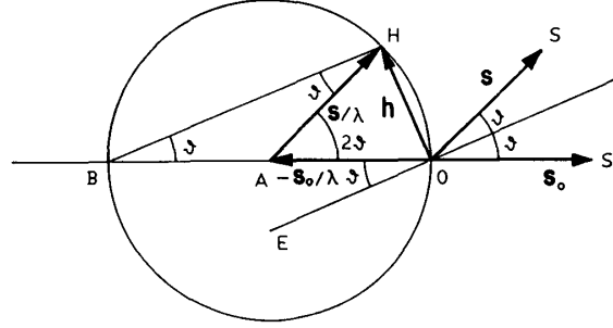
Fig. 4. Schematic representation of Laue condition and Ewald's sphere.
