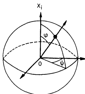
Fig. 12. Spherical coordinate specifying polar angle \phi and azimuthal angle \psi of a plane-normal with respect to a reference axis X_i .
