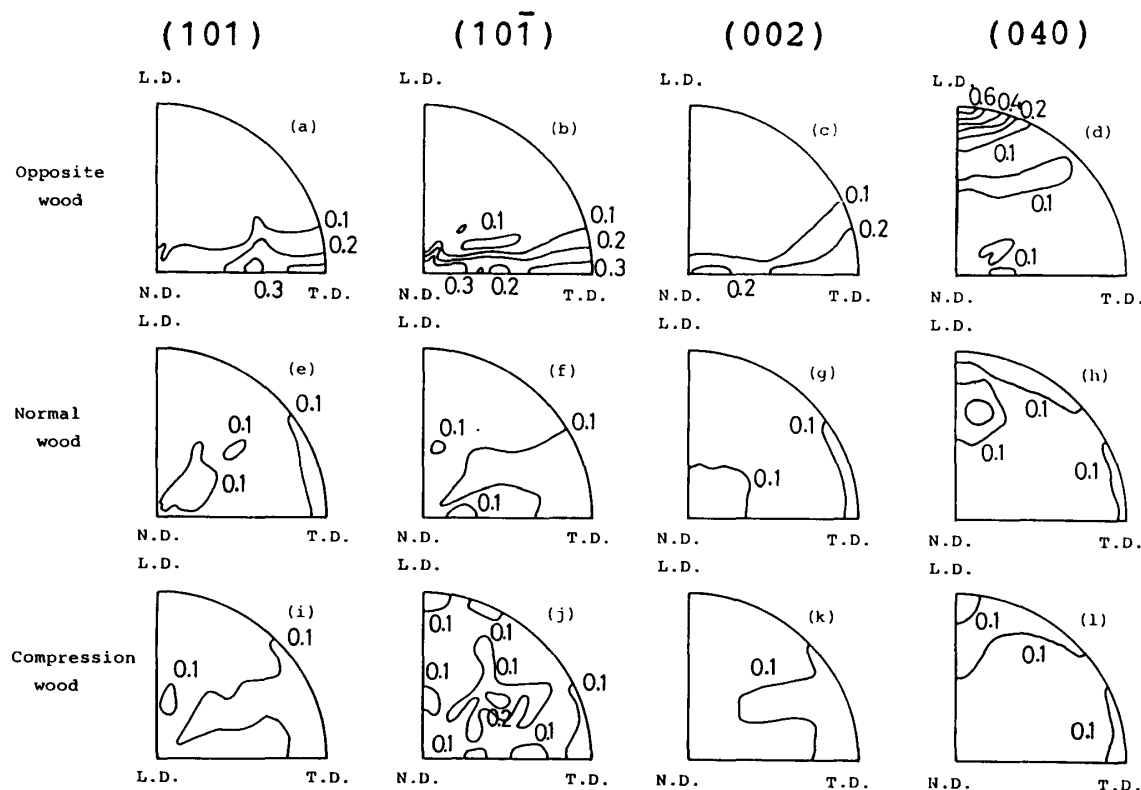
Fig. 28. Pole figure diagrams for cellulose crystallites in Pinus densiflora wood expressed by probability functions.
