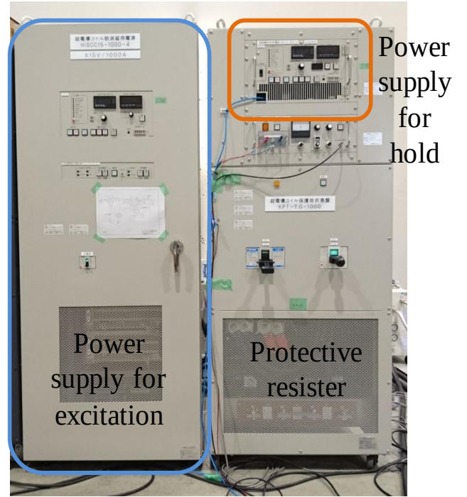
Fig. 2. Highly stabilized power supply for HTS-MRI magnet. Power supply for excitation is on the left and power supply for hold is on the upper right.
