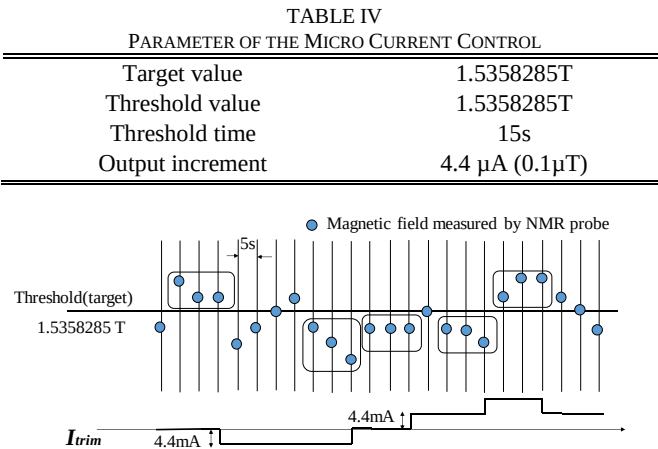
Fig. 4. Control scheme of the micro current control.
