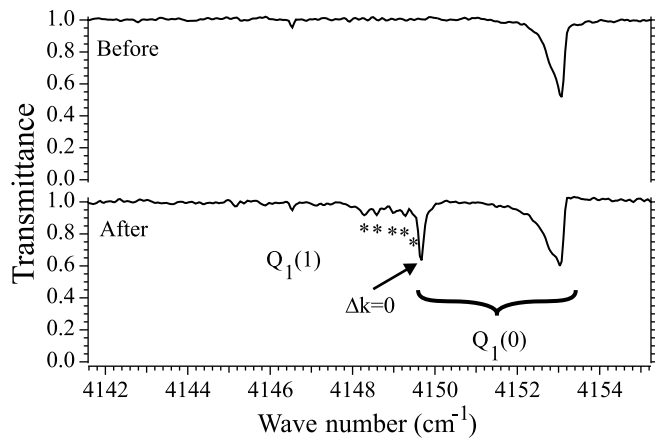
FIG. 1. Low resolution ( \Delta\nu \sim 0.1 \text{ cm}^{-1} ) spectrum of a parahydrogen crystal before (the upper trace) and after (the lower trace) the \gamma -ray irradiation observed by a BOMEM DA-2 FTIR spectrometer. Only the spectral region around the Q_1(0) transition is shown. The prominent spectral line marked with the arrow is due to the \Delta k = 0 vibron transition induced by the macroscopic Gauss electric field due to the imbalance of positive and negative charges. The lines marked with asterisks are the Stark shifted infrared absorption of hydrogen molecules close to charges.
