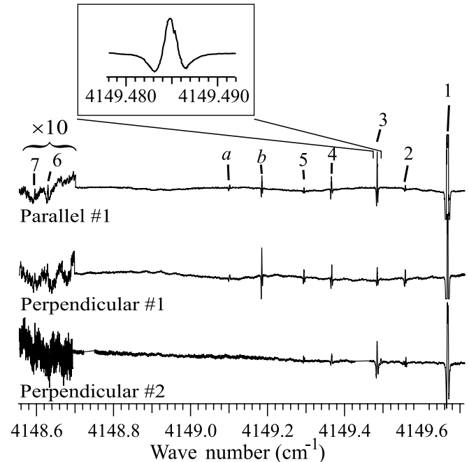
FIG. 2. High resolution spectrum of two different (No. 1 and No. 2) \gamma -ray irradiated parahydrogen crystals. Tone-burst modulation with sidebands of 48 MHz was used to record each spectrum. The upper and middle traces show the absorption of crystal No. 1 with the polarized radiation oriented parallel and perpendicular to the c axis, respectively. The lower trace shows the absorption of crystal No. 2 with polarization perpendicular to the c axis. While several lines are observed in both polarizations due to imperfections in the optical system, the large differences in intensities for different polarization demonstrate the existence of well defined selection rules. The labels in the figure correspond to those given in Table I. The inset is the expansion of lines at 4149.4848 \text{cm}^{-1} .
