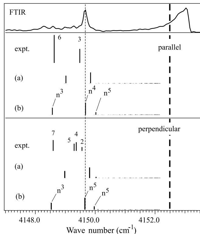
FIG. 3. Stick diagrams of the experimentally observed spectrum (expt.) and the calculated spectrum [(a) and (b)] for parallel (middle panel) and perpendicular (lower panel) polarizations. The experimental lines are labeled as in Fig. 2 and Table I. The stick diagrams (a) in each panel show the calculated spectra with the assumption of a rigid hcp structure, while diagrams labeled (b) are the calculated spectra with the assumption of a 5% isotropically shrunk hcp structure. The symbols n^3 , n^4 , and n^5 in the diagrams (b) are the transitions of hydrogen molecules next-nearest neighbor, next-next-nearest neighbor, and next-next-next-nearest neighbor to an ion, respectively. The intensities of the observed spectrum were measured by integrating the spectral profile taken from the unmodulated absorption spectrum. They are different from the intensities measured in tone-burst modulation which intensifies sharp lines. The vertical broken line at 4149.67 \text{ cm}^{-1} shows the position of the \Delta k = 0 transition. The bold broken line at 4152.50 \text{ cm}^{-1} shows the origin of the Q_1(0) transition from which the spectral lines are Stark shifted. The upper panel gives the FTIR absorption spectrum from Fig. 1.
