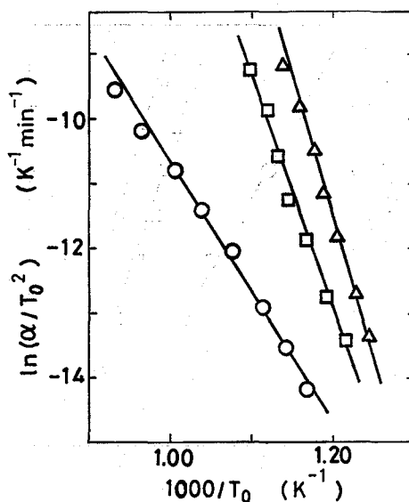
Fig. 8. Kissinger plot of data obtained from DTA curves of \text{Li}_2\text{O}-2\text{SiO}_2 glass ( n=m=1 )
