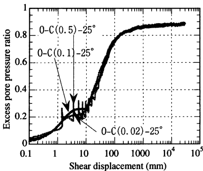
Fig. 19 The residual pore pressure ratios of O-samples in CU-C tests with different frequencies.
