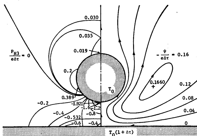
Fig. 5. Streamlines and isobars. ( h=r-d=2 , r \rightarrow \infty , d \rightarrow \infty ; the arrows show the direction of flow for \Delta\tau > 0 .)
