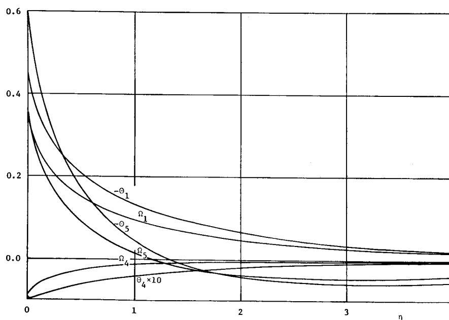
Fig. 10. Knudsen-layer functions II.
